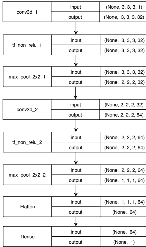
Figure 12: Structure of the convolutional neural network used (set of TensorFlow routines).
