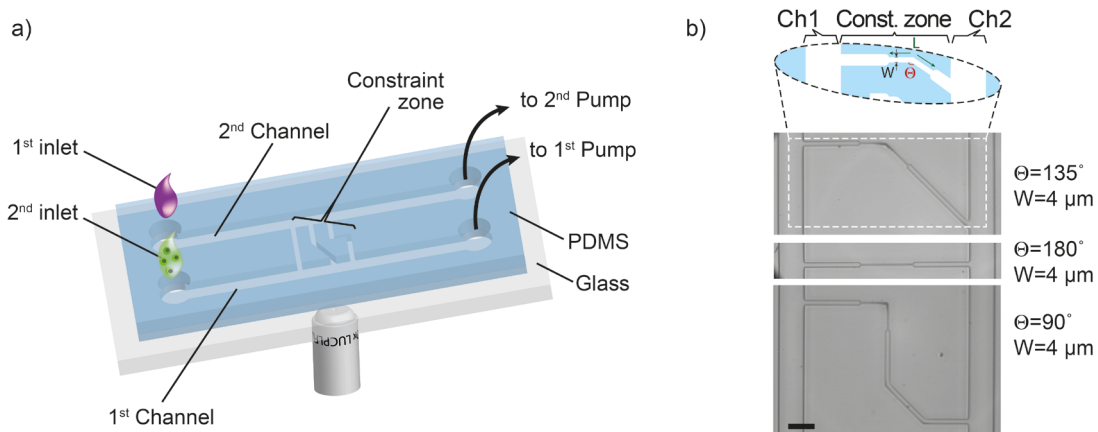
Figure 1: a) Overall view of the microfluidic device with two parallel channels and constraints connecting them. b) Different constraint geometries in a fabricated device to analyze the glioma migration. Scale bar: 100 \mu\text{m} .
