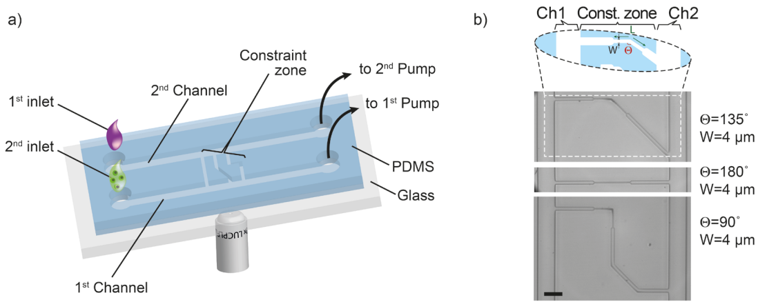
Figure 1: a) Overall view of the microfluidic device with two parallel channels and constraints connecting them. b) Different constraint geometries in a fabricated device to analyze the glioma migration. Scale bar: 100 \mu\text{m} .
