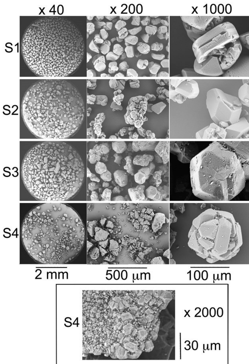
Figure 1. Scanning electron microscopy photographs of crystalline C_{60} powders of samples S1, S2, S3, and S4 with different magnifications. The inset shows the photograph of an aggregate of C_{60} crystals found in sample S4.
