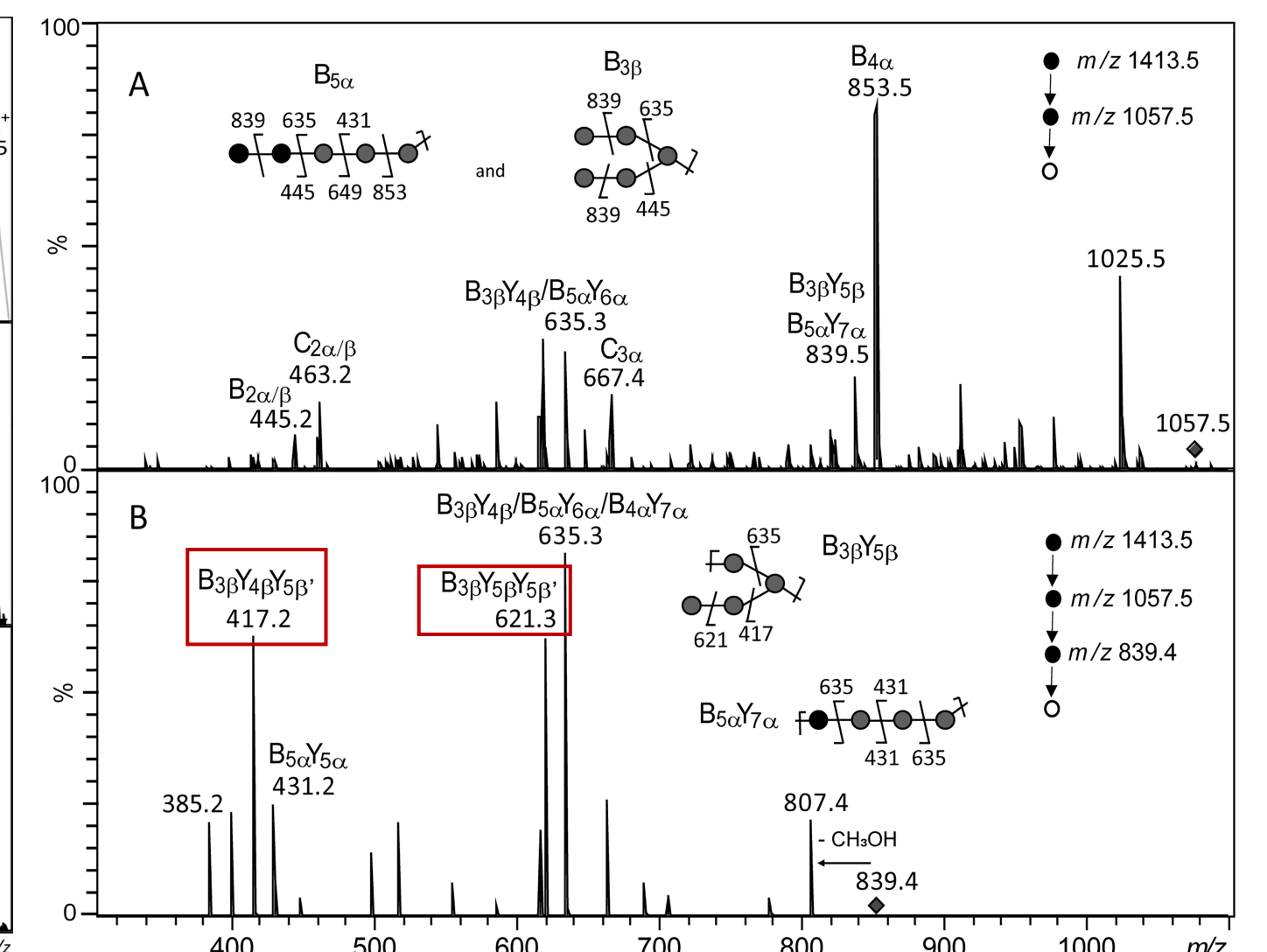
Fig. 4 : Multistage tandem mass spectrometry analysis allowing the determination of the structure of the permethylated LLO-released oligosaccharide isolated from the diatom P. tricornutum .
