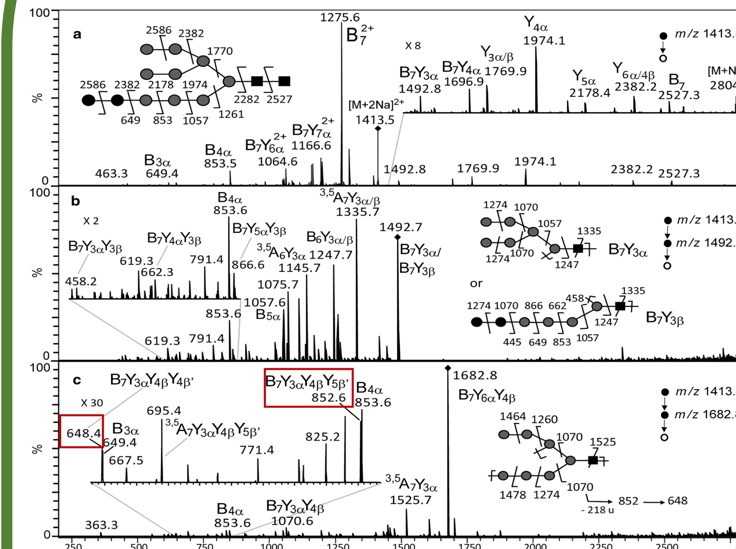
Fig. 3 : Multistage tandem mass spectrometry analysis allowing the determination of the structure of the permethylated LLO-released oligosaccharide isolated from the diatom P. tricornutum .
