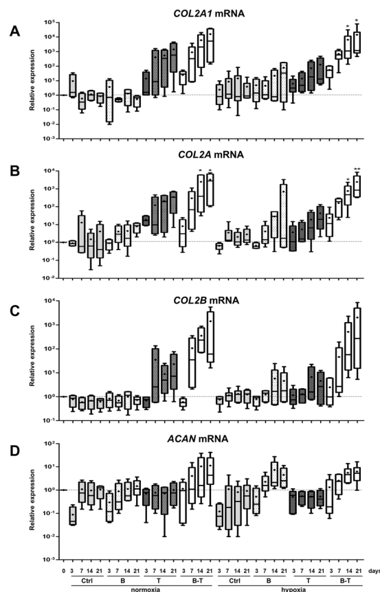
Figure 3. Effects of oxygen tension, BMP-2 and/or TGF-β1 on the mRNA levels of specific cartilage markers. hBM-MSCs were cultured in type I collagen sponges for 3, 7, 14, and 21 days under normoxia or hypoxia, in the absence (Ctrl), or presence of 50 ng/mL BMP-2 (B), 10 ng/mL TGF-β1 (T), or both (B-T). The steady-state mRNA levels for type II collagen were measured using real time RT-PCR with primers or probe specific for type IIA collagen ( COL2A mRNA) (B), type IIB collagen ( COL2B mRNA) (C), or the total amount of type IIA and IIB collagen ( COL2A1 mRNA) (A). The levels of mRNA encoding aggrecan ( ACAN mRNA) were also evaluated with specific primers (D). All results were normalized to RPL13a mRNA and are presented as the expression of each gene relative to that of undifferentiated hBM-MSCs at day 0. Box plots represent independent experiments performed in triplicate (n = 4). Statistically significant differences between the undifferentiated cells at day 0 and treated cells are presented and were determined using the Kruskal-Wallis test (*P < 0.05, **P < 0.01).
