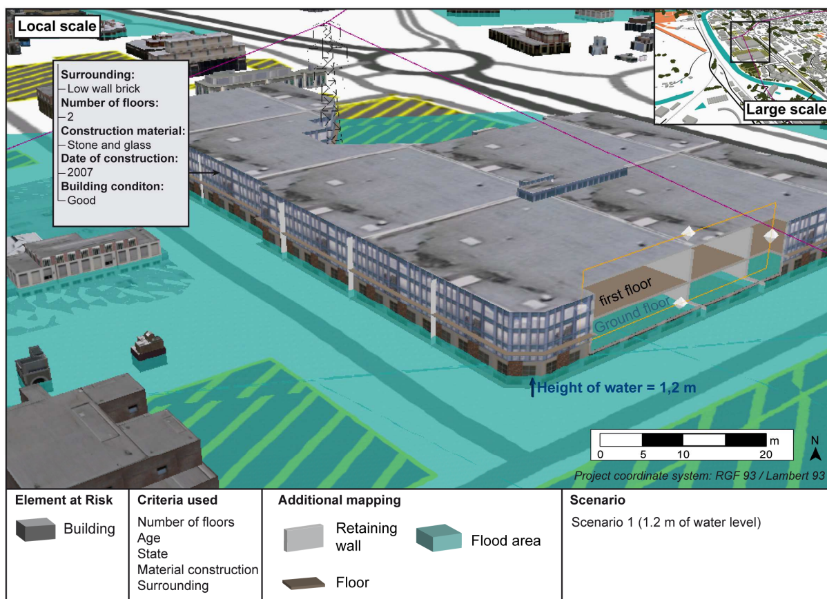
Fig. 11. EaRs identified in flood zone areas for a 1.2 m water level at the local scale.
