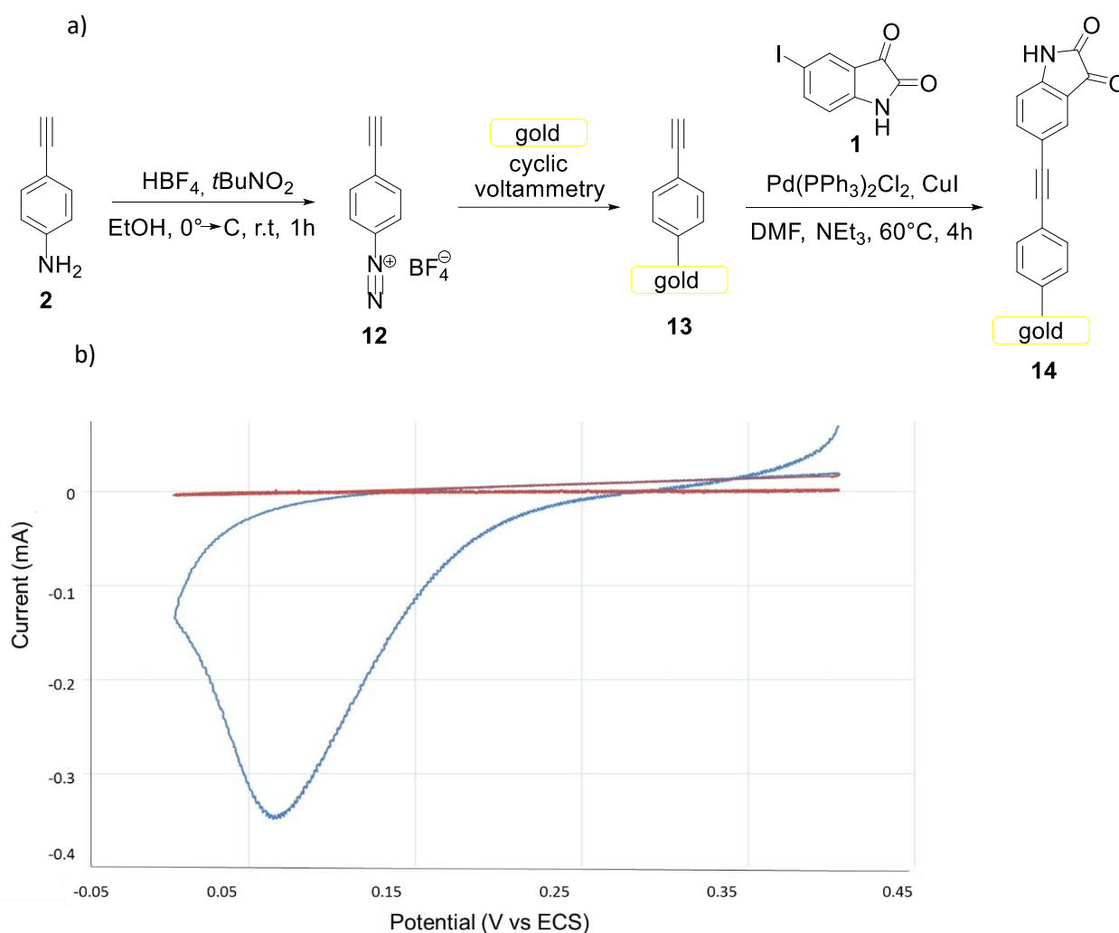
Fig. 6. a) Grafting of compound 1 on activated gold surface 13 and b) the electroreduction by cyclic voltammetry ( 100 \text{ mV}\cdot\text{s}^{-1} ) of diazonium 12 . Blue and red curves correspond to first and second cycle respectively.
