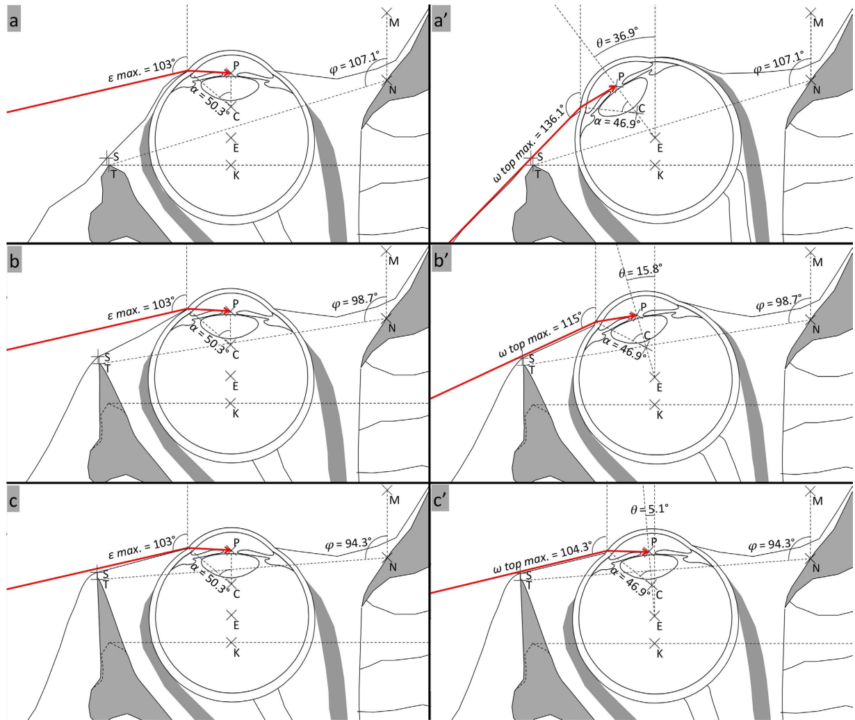
Figure 3. Schematic cross-sections illustrating \varepsilon_{\text{max}} and \omega_{\text{top max.}} values for the human orbit and two modified non-human ape-like orbits. Schematic cross-sections of the Human orbit (a and a'; \varphi = 107.1^\circ ), modified “Pan-like” orbit (b and b'; \varphi = 98.7^\circ ), and modified “Gorilla-like” orbit (c and c'; \varphi = 94.3^\circ ). In a, b and c, the eye is in primary position of gaze. The \varepsilon_{\text{max}} value is 103^\circ for each orbit type. In a', b', c', the eye is in the abduction position (denoted by \theta ) that yields the \omega_{\text{top max.}} value. In the human orbit, \omega_{\text{top max.}} is 136.1^\circ for 36.9^\circ abduction. In the modified “Pan-like” orbit, \omega_{\text{top max.}} is 115^\circ for 15.8^\circ abduction. In the modified “Gorilla-like” orbit, \omega_{\text{top max.}} is 104.3^\circ for 5.1^\circ abduction.
