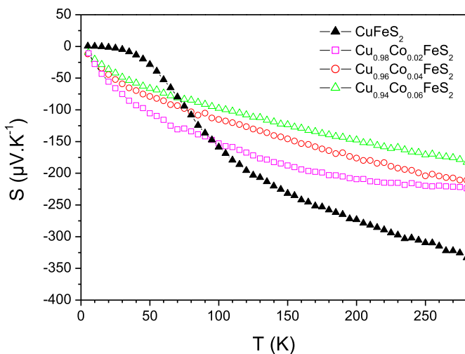
Fig. 6. T dependence of S measured at low temperature on samples prepared by solid state reaction and cold pressed.
