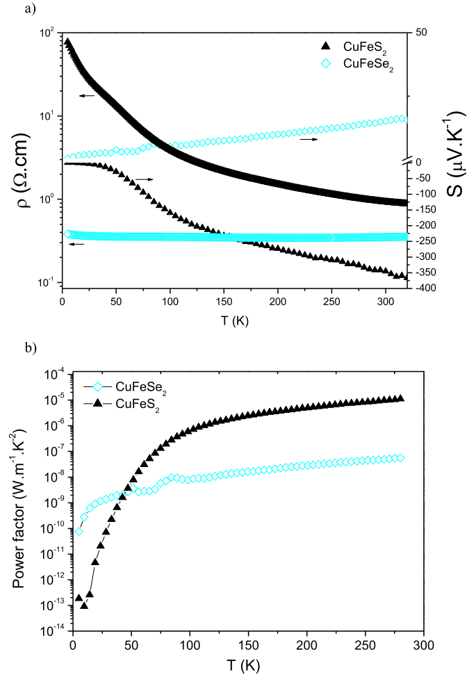
Fig. 4. (a) Temperature ( T ) dependence of the electrical resistivity ( \rho ), left y-axis and Seebeck coefficient ( S ), right y-axis of \text{CuFeS}_2 and \text{CuFeSe}_2 measured at low temperature (b) T dependence of the power factor of \text{CuFeS}_2 and \text{CuFeSe}_2 measured at low T .
