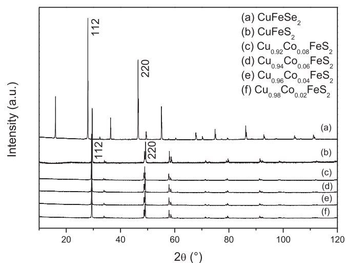
Fig. 2. Powder diffraction patterns of \text{CuFeS}_2 samples obtained after solid state reaction. hkl index are given for the main peaks of both structure type.
