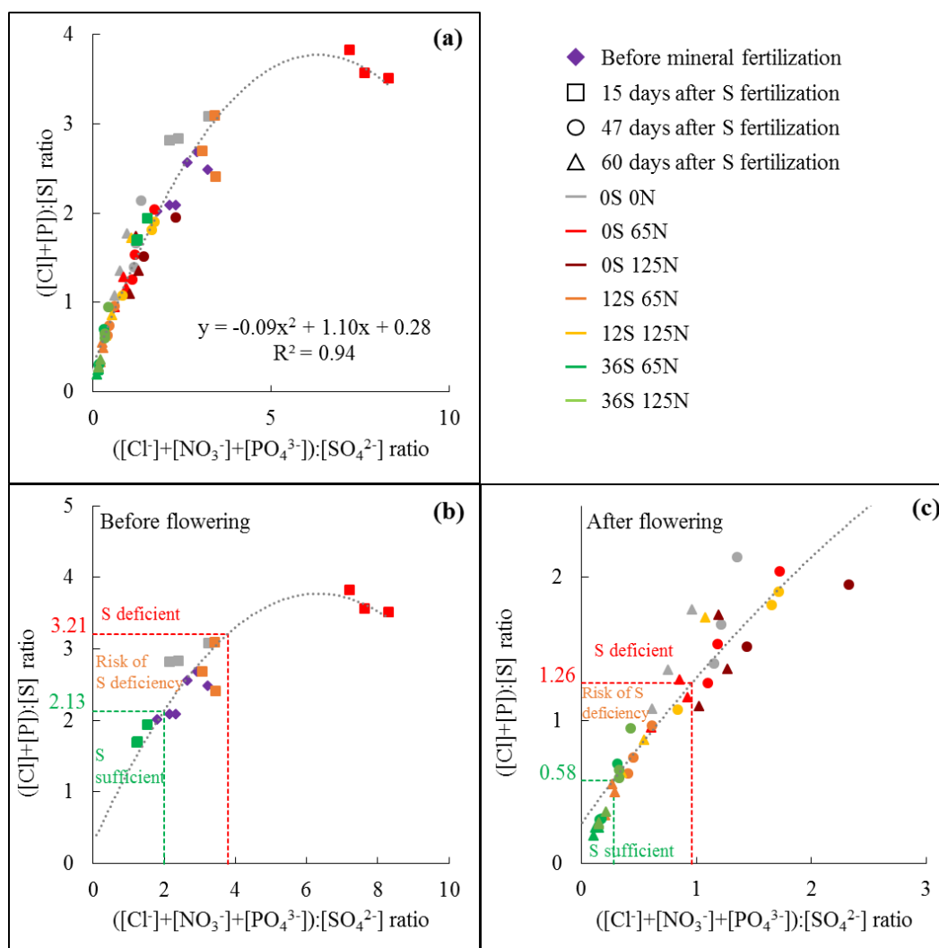
Figure 3. Correlation between the ([Cl^-]+[NO_3^-]+[PO_4^{3-}]):[SO_4^{2-}] ratio and the ([Cl^-]+[P]):[S] ratio in mature leaves of oilseed rape submitted to different N and S fertilization rates (field experiment 1), (a) for all data points (all fertilization treatments, leaves harvested before mineral fertilization, or 15, 47 or 60 days after S fertilization), or for mature leaf samples harvested (b) before or (c) after flowering. Thresholds of the ([Cl^-]+[P]):[S] ratio were determined as the difference or sum between the mean and the 95% confidence interval of plants receiving 0 or 36 kg S ha -1 , defining three groups of plants: S deficient, at risk of S deficiency and S sufficient plants.
