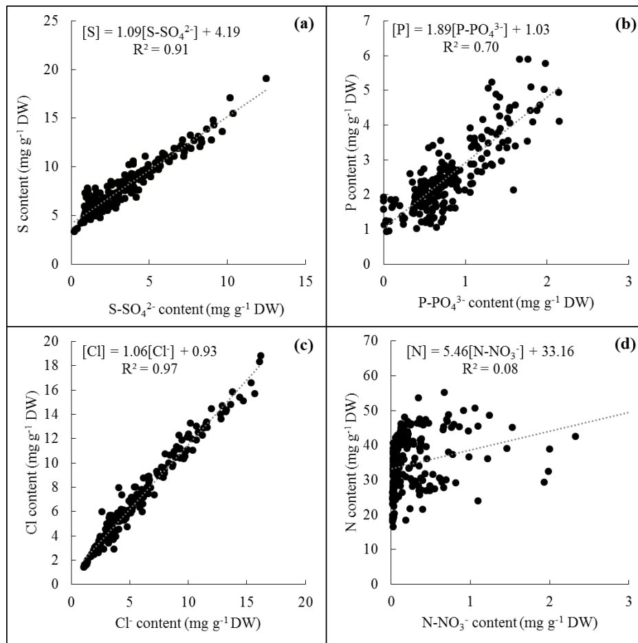
Figure 2. Correlation between (a) S- \text{SO}_4^{2-} and S content ( \text{mg g}^{-1} \text{ DW} ); (b) P- \text{PO}_4^{3-} and P content ( \text{mg g}^{-1} \text{ DW} ); (c) \text{Cl}^- and Cl content ( \text{mg g}^{-1} \text{ DW} ) and (d) N- \text{NO}_3^- and N content ( \text{mg g}^{-1} \text{ DW} ). Ion contents were quantified by HPLC and element contents by X-ray fluorescence (XRF), except N which was quantified by IRMS, in leaves of oilseed rape grown under field conditions (field experiment 1 and the second part of field experiment 2). Data used were obtained from plants of all fertilization treatments.
