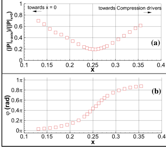
Fig. 11: (a) |P'_{x,0.025}|/|P'_{0.5,0.025}|_{\max} ; (b) \varphi(f_r, x) . f_r = 600 Hz, L_c = 0.8 m, w/o flames.
