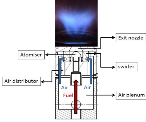
Fig. 2: Injector with a two-phase flow swirling flame.
