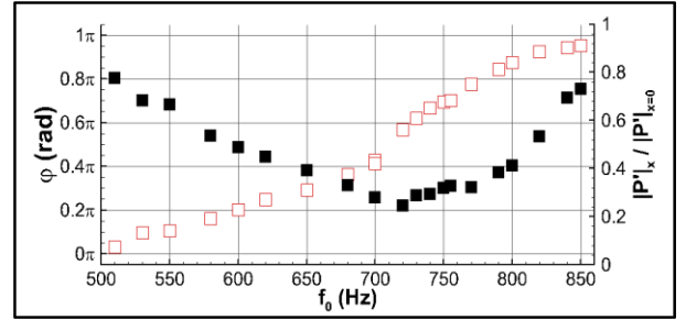
Fig. 13: |P'_{0.256,0,z}|/|P'_{0,0,z}| (■), \varphi(f_0, x = 0.256) (□). L_c = 0.8 m, with flames.
