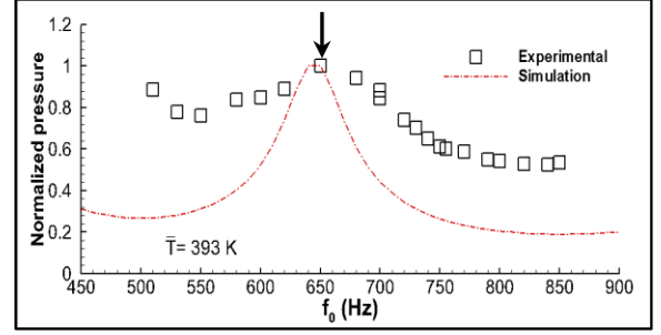
Fig. 12: |P'_{0,y,z}|/|P'_{0,y,z}|_{\max} vs. f_0 . Arrow: f_r = 650 Hz. L_c = 0.8 m, with flames.
