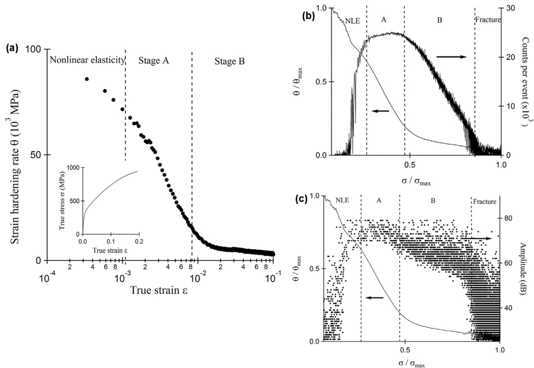
Fig. 3. (a) Typical work hardening curve for polycrystalline cobalt and corresponding tensile curve in insert. (b) Relative strain hardening rate \theta/\theta_{max} and counts per event depicted by acoustic emission versus relative stress level \sigma/\sigma_{max} . (c) Relative strain hardening rate \theta/\theta_{max} and amplitude variation of acoustic emission versus relative stress level \sigma/\sigma_{max} .
