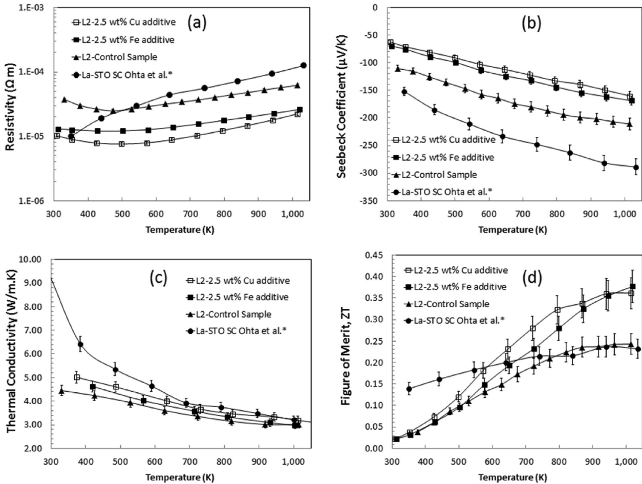
Fig. 5. Thermoelectric properties of the \text{Sr}_{0.8}\text{La}_{0.06}\text{Ti}_{0.8}\text{Nb}_{0.2}\text{O}_3 (control) and the Cu-containing and Fe-containing samples as a function of temperature: (a) electrical resistivity, (b) Seebeck coefficient, (c) thermal conductivity, (d) figure of merit, ZT. Data for doped single crystal \text{SrTiO}_3 (round solid symbols; taken from Ohta et al. [51]) are included for comparison.
