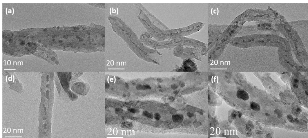
Figure 2. TEM images of the CNT confined iron catalysts under different calcination temperature.
