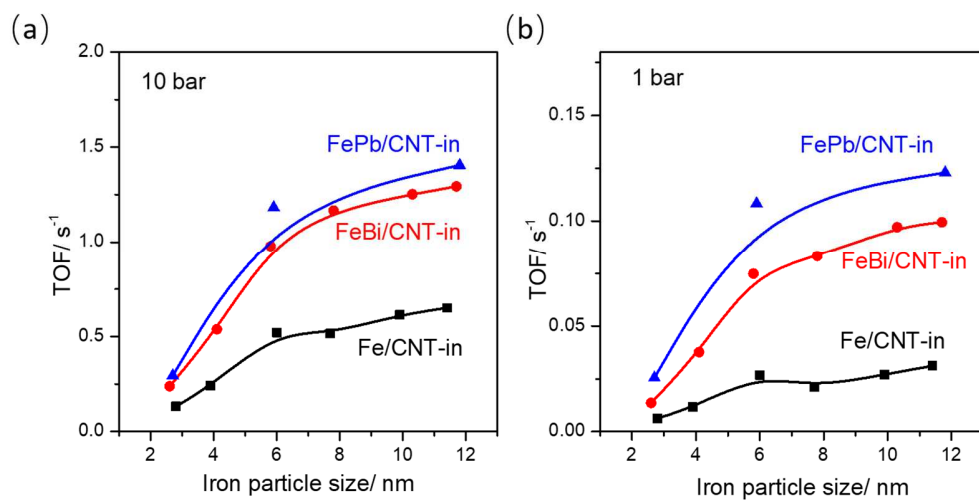
Figure 11. Iron particle size effect on the TOF (350 °C, H_2/CO = 1/1 , GHSV = 17 L/g.h (10bar) or 3.4 L/g.h (1bar), TOS = 10 h).
