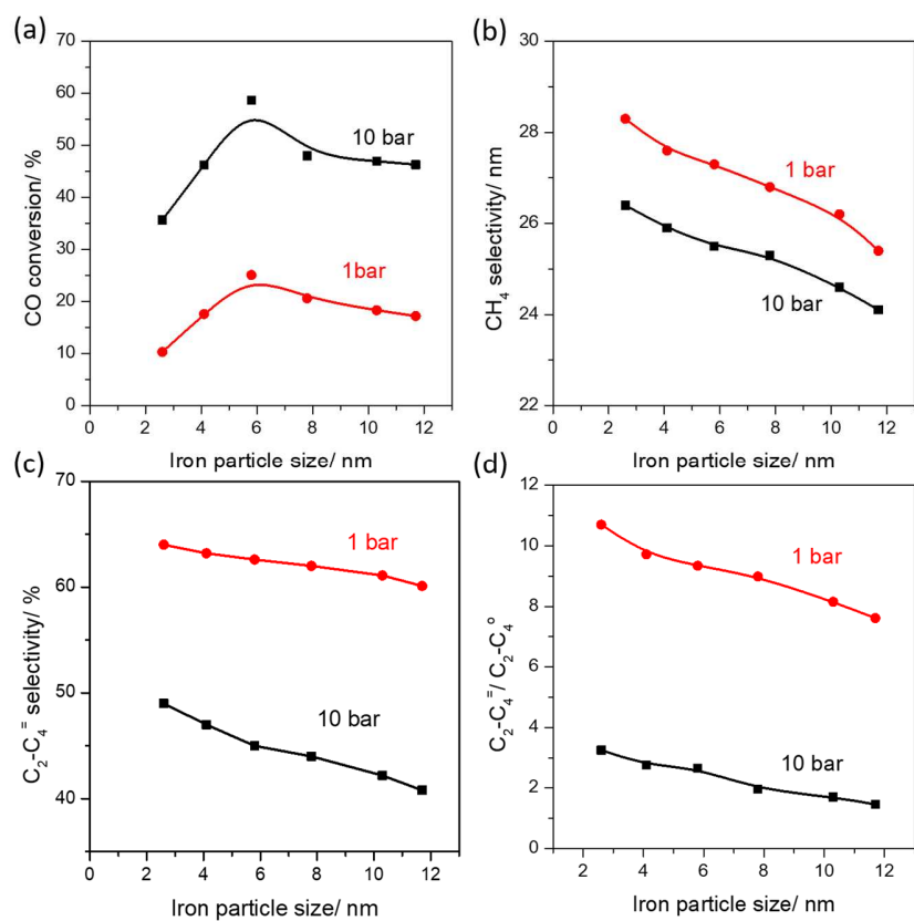
Figure 9. CO conversion and product selectivity versus iron particle size over Bi promoted iron catalysts. (350 °C, H 2 /CO = 1/1, GHSV = 17 L/g.h (10bar) or 3.4 L/g.h (1bar), TOS = 10 h).
