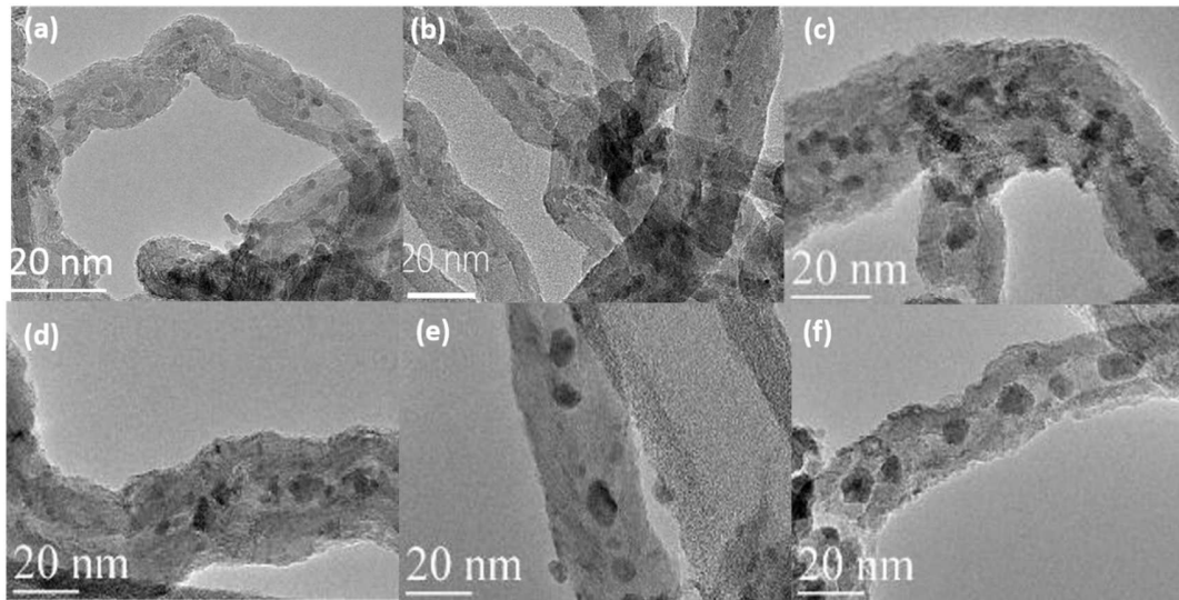
Figure 4. TEM images of the CNT confined iron catalysts promoted with Bi under different calcination temperature. (a) FeBi/CNT-in-300, (b) FeBi/CNT-in-350, (c) FeBi/CNT-in-400, (d) FeBi/CNT-in-450, (e) FeBi/CNT-in-500, (f) FeBi/CNT-in-600.
