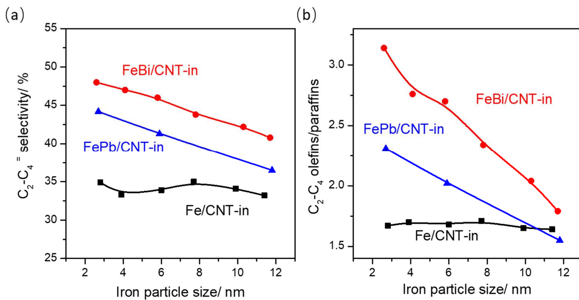
Figure 8. C 2 -C 4 olefin selectivity and olefin to paraffin ratio as function of the size of iron nanoparticles confined in CNT at CO conversion of 40-50%. The reaction condition: 350 °C, H 2 /CO = 1/1, GHSV = 10.2-23.8 L/g.h, P=10 bar, TOS = 10 h.
