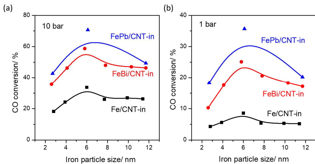
Figure 10. Iron particle size effect on the CO conversion over Bi or Pb promoted and unpromoted iron catalysts (350 °C, H 2 /CO = 1/1, GHSV = 17 L/g.h (10bar) or 3.4 L/g.h (1bar), TOS = 10 h).
