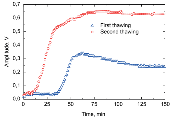
Fig. 13. Evolution of the peak-to-peak voltage of the signal reflected by a sample of salmon
