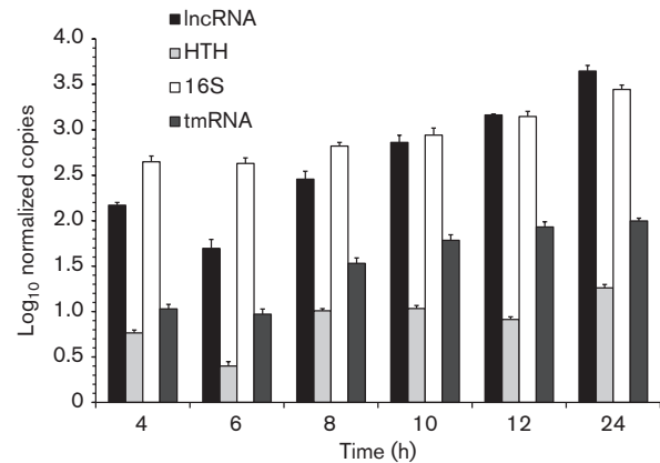
Fig. 2. Expression level of the lncRNA during the growth of L. salivarius UCC118. The expression levels of lncRNA (LSL 1885 and tail), HTH (LSL 1884 ), 16S rRNA and tmRNA were quantified by RT-qPCR after 4, 6, 8, 10, 12 and 24 h of a L. salivarius UCC118 culture. Data are means \pm SD of four independent replicates.
