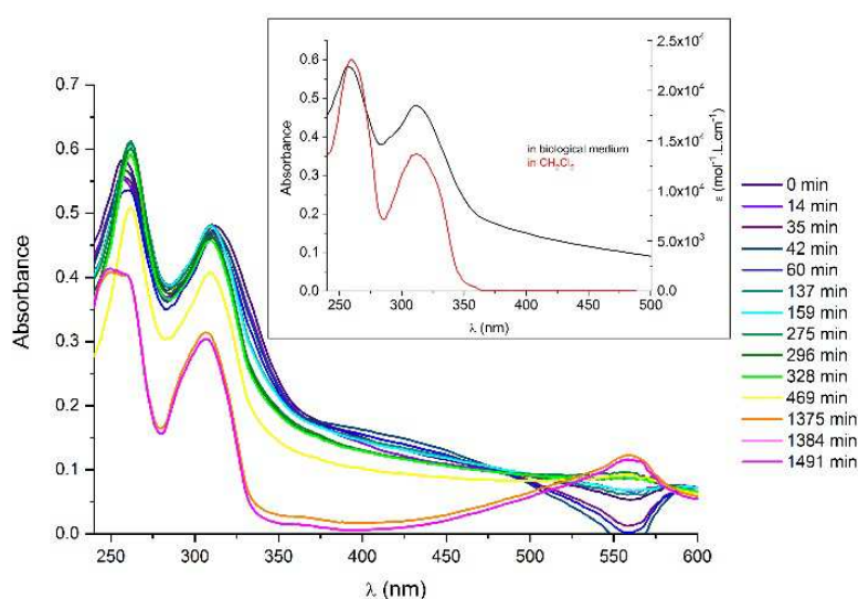
Figure 2. Stability of 12 followed by UV-vis spectroscopy over 25 h in 1% DMSO/DMEM+GlutaMAX-I TM solution ( c = 50 \mu\text{M} ) and UV-visible spectra of 12 in dichloromethane solution ( c = 100 \mu\text{M} ) (red line, inset) and in 1% DMSO/DMEM+GlutaMAX-I TM solution ( c = 50 \mu\text{M} ) in absence of cell line (dark line, inset).
