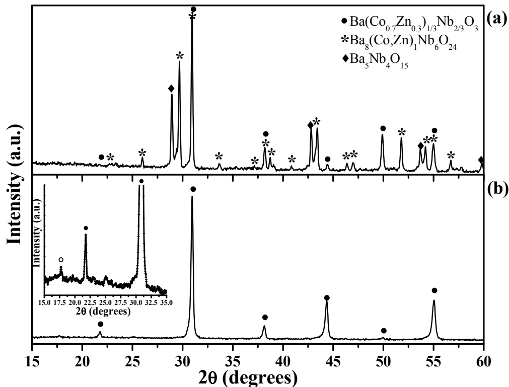
Figure 5. X-ray diffractograms of a BCZN ceramic (S2a): (a) at the upper surface and (b) at a depth of 140 \mu\text{m} below the surface. ●: \text{Ba}(\text{Co}_{0.7}\text{Zn}_{0.3})_{1/3}\text{Nb}_{2/3}\text{O}_3 ; *: \text{Ba}_8(\text{Co,Zn})_1\text{Nb}_6\text{O}_{24} ; ◆: \text{Ba}_5\text{Nb}_4\text{O}_{15} . Inset: The region limited between 15^\circ and 35^\circ 2\theta shows a superlattice peak for 1:2 ordering denoted by an open circle.
