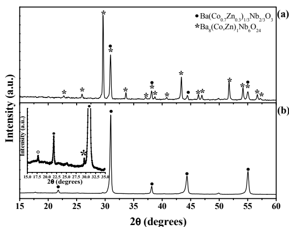
Figure 3. X-ray diffractograms of a BCZN ceramic (S1a): (a) at the upper surface and (b) at a depth of 120 \mu\text{m} below the surface. ●: \text{Ba}(\text{Co}_{0.7}\text{Zn}_{0.3})_{1/3}\text{Nb}_{2/3}\text{O}_3 ; *: \text{Ba}_8(\text{Co,Zn})_1\text{Nb}_6\text{O}_{24} . Inset: The region limited between 15^\circ and 35^\circ 2\theta shows a superlattice peak for 1:2 ordering which is denoted by an open circle.
