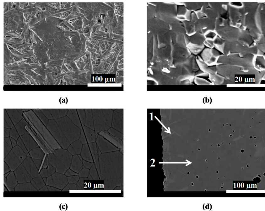
Figure 7. SEM micrographs of BCZN ceramics (S1a): (a) of a surface; (b) of a fractured surface; (c) of a grain boundary; and (d) of a longitudinally polished section.
