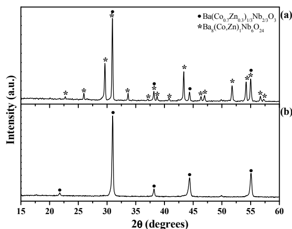
Figure 2. X-ray diffractograms of a BCZN ceramic (S1): (a) at the upper surface and (b) at a depth of 90 \mu\text{m} below the surface. ●: \text{Ba}(\text{Co}_{0.7}\text{Zn}_{0.3})_{1/3}\text{Nb}_{2/3}\text{O}_3 ; *: \text{Ba}_8(\text{Co,Zn})_1\text{Nb}_6\text{O}_{24} .
