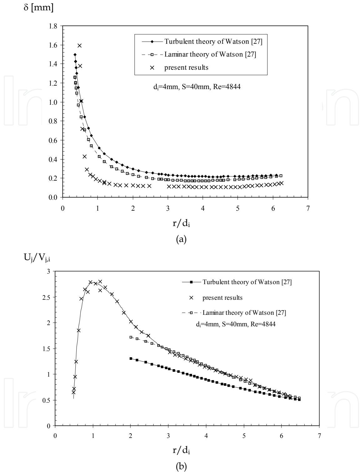
Fig. 8. Comparison of the experimental results with Watson’s theory: (a) liquid layer depth (b) dimensionless radial mean velocity.
