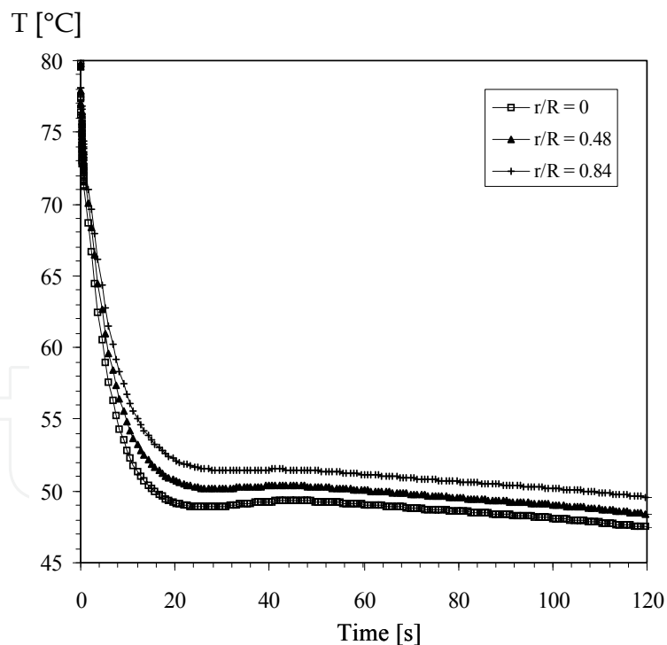
Fig. 13. Temperatures inversely predicted at the top surface.
