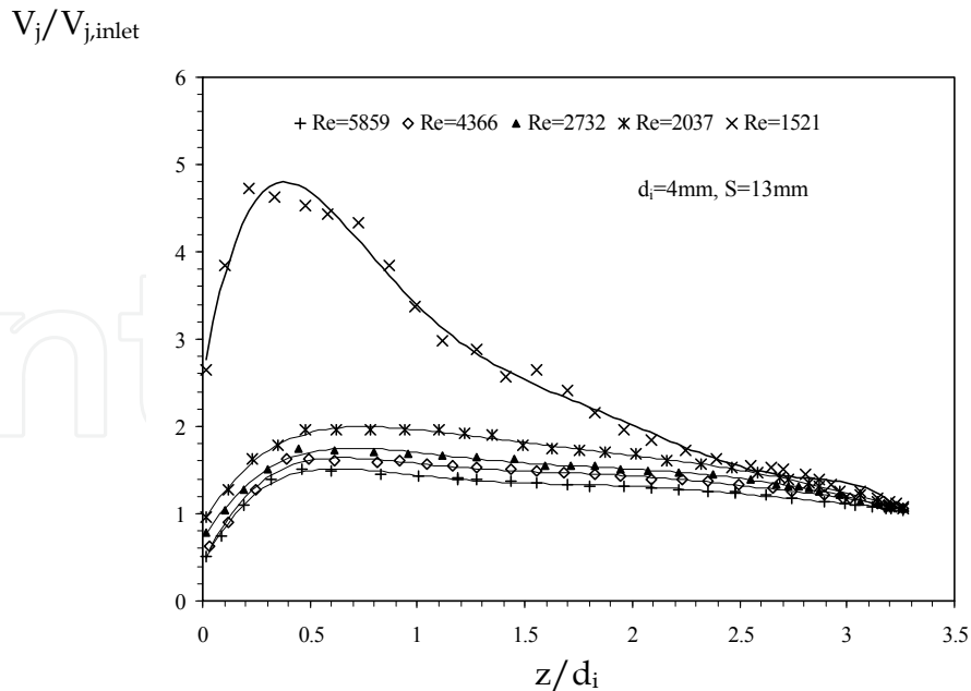
Fig. 4. Dimensionless axial velocity of the jet.
