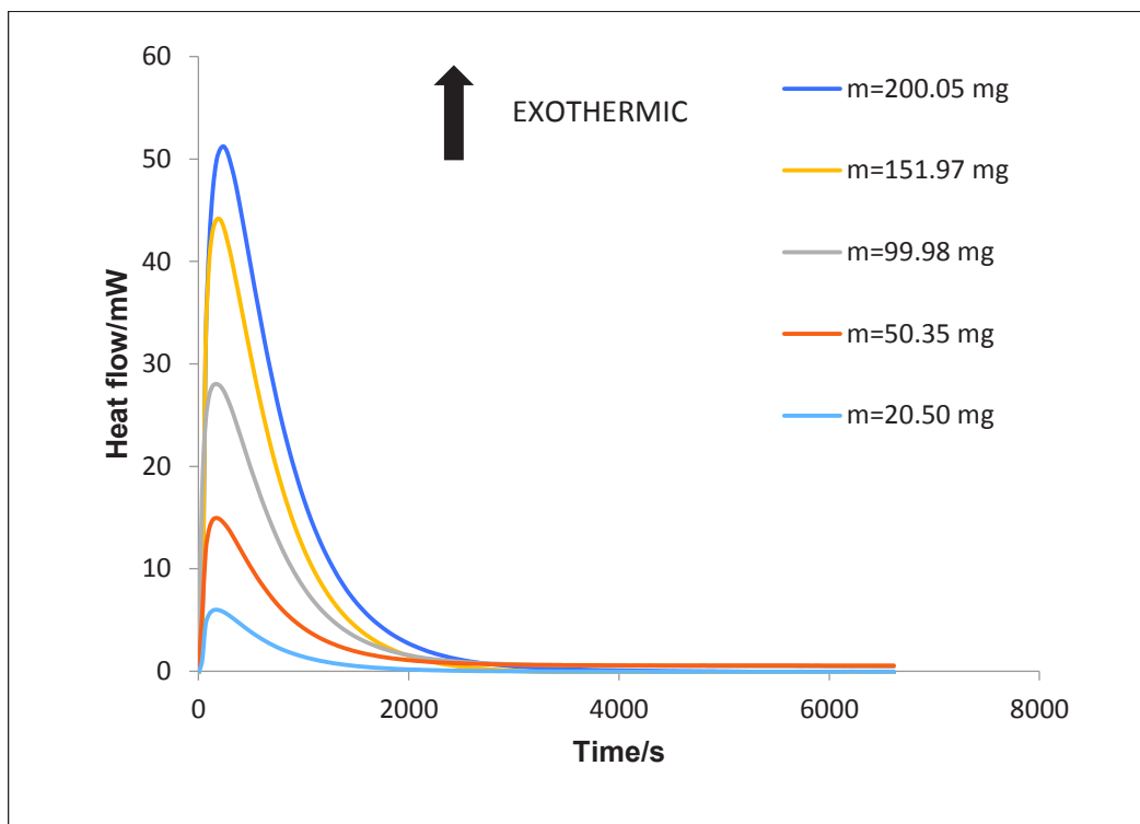
Fig.7 Dissolution of the low phosphate PK1 in the solution S1 at 25°C at different sample mass.
