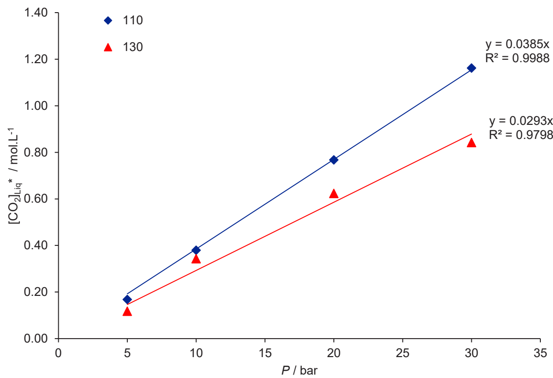
Figure S11. Evolution of the solubility of CO 2 at different CO 2 pressure for EFAME
