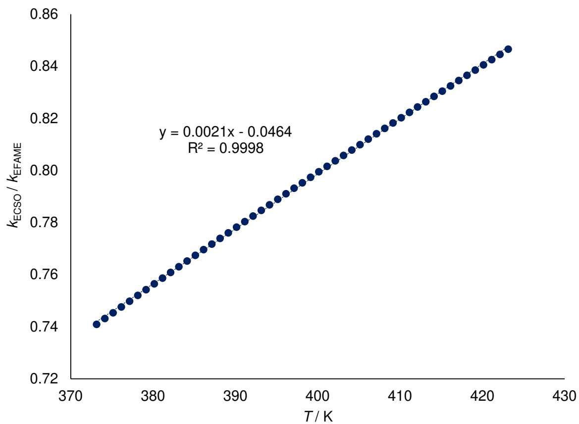
Figure 12. The variation of \frac{(k_{\text{carbonation}})_{ECISO}}{(k_{\text{carbonation}})_{EFAME}} with different reaction temperature.
