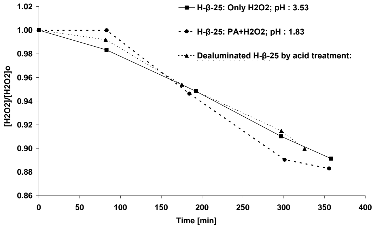
Fig. 1 Experiments carried out in the presence of H-β-25 zeolite at 50°C, at 350 rpm and loading of 18.25 g/l
