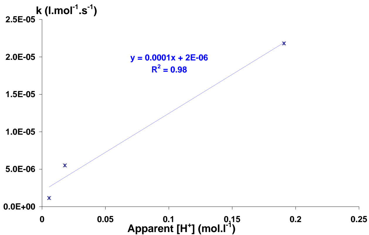
Fig. 7 Rate constants versus apparent [\text{H}^+]
