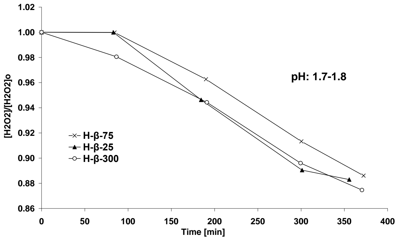
Fig. 3 Experiments carried out with a mixture of PA and H 2 O 2 over H-β zeolites at 50°C, at 350 rpm and loading of 18.25 g/l
