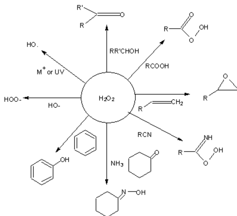
Scheme 1. Applications of H_2O_2 in fine chemical reactions
