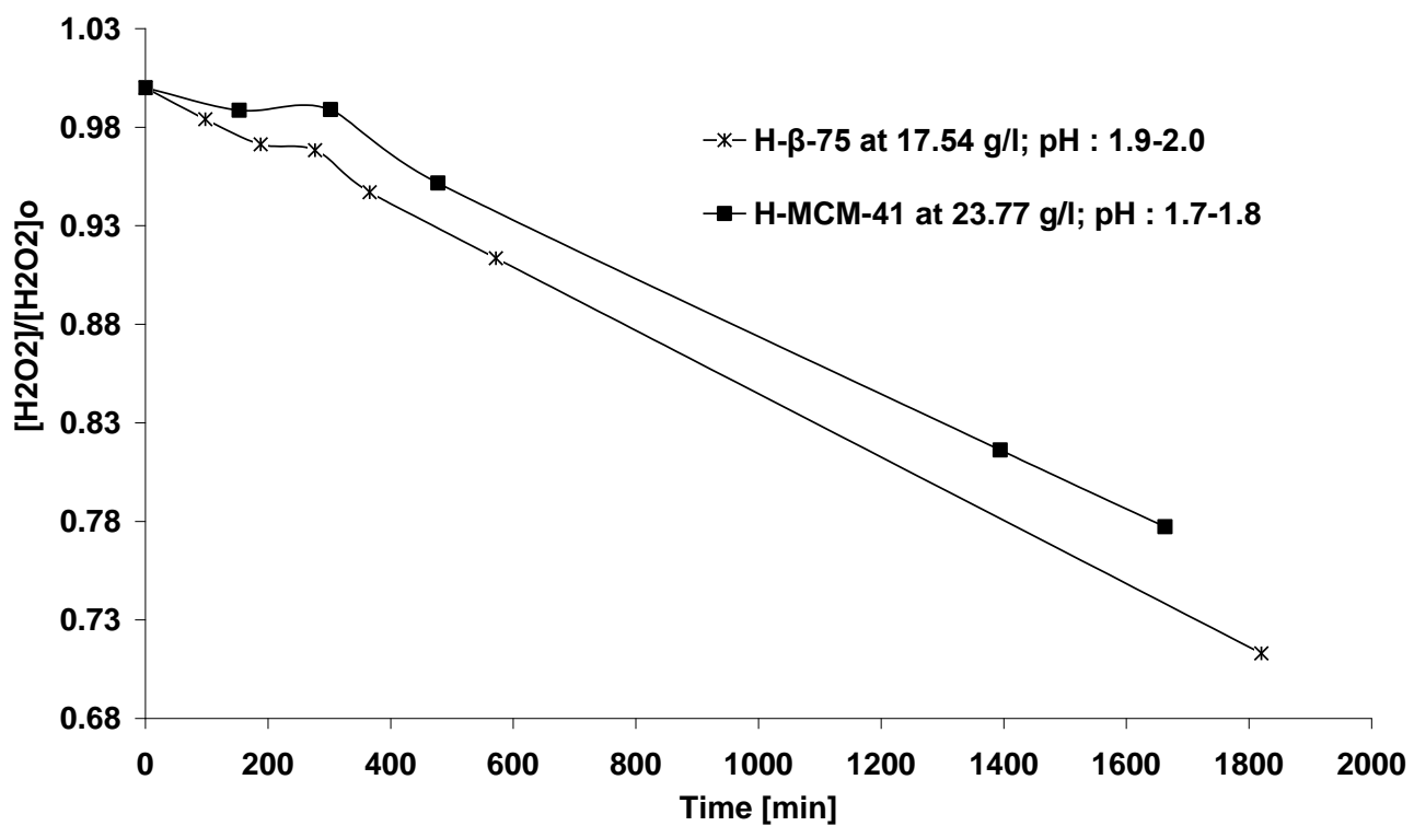
Fig. 5 Experiments carried out with a mixture of PA and H 2 O 2 over H-MCM-41 and H- \beta -75 at 40°C and at 350 rpm
