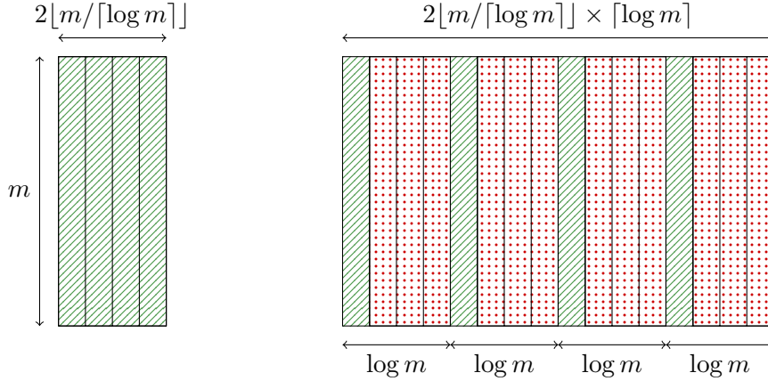
Figure 5: Reshaping CANDIDATE into PROPER
