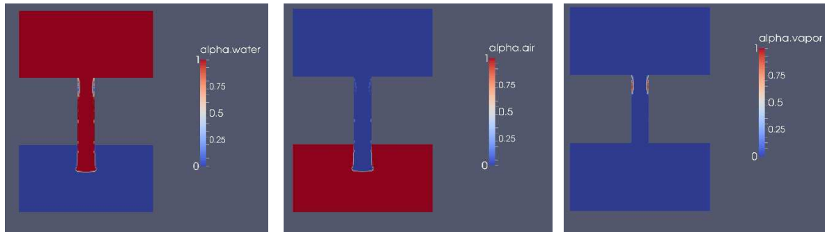
Figure 2. Simulation of cavitating injection: liquid, vapour and air volume fraction fields
