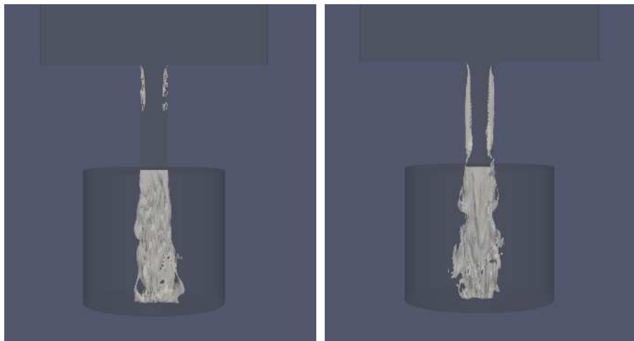
Figure 1. Simulations of the Sou's experiments. Cavitation number of 0.94 (left) and 0.65 (right)
