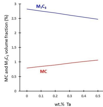
Figure 2b: Volume fractions (vol. %) of M_7C_3 and MC carbides as predicted by thermocalc at 1200^\circ\text{C} for the FeCrNi alloys of the present study and plotted as a function of the Ta concentration (wt.%)
