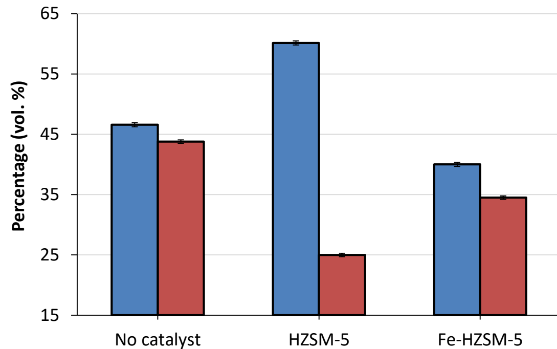
(b) Xylan
