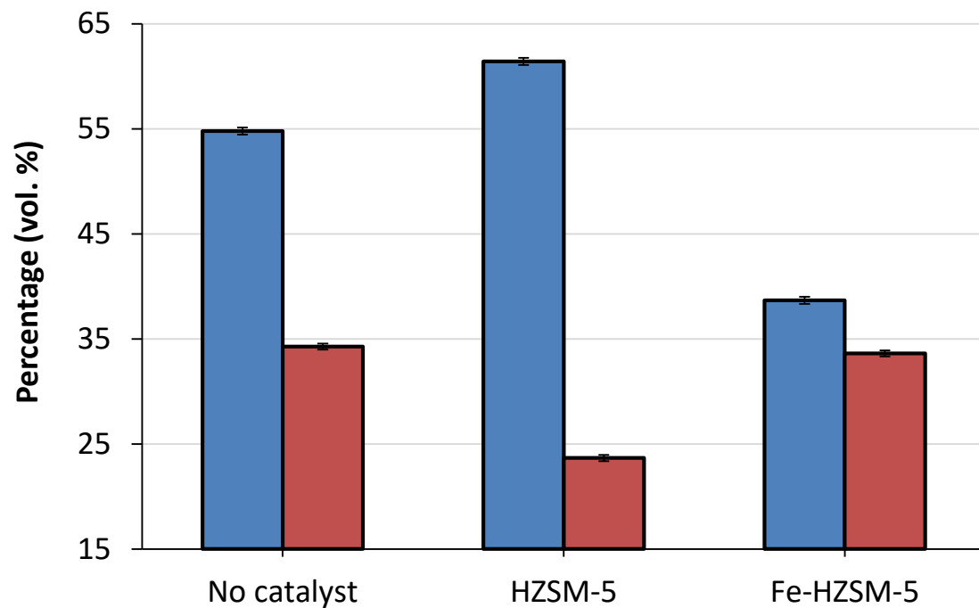
(a) Cellulose
