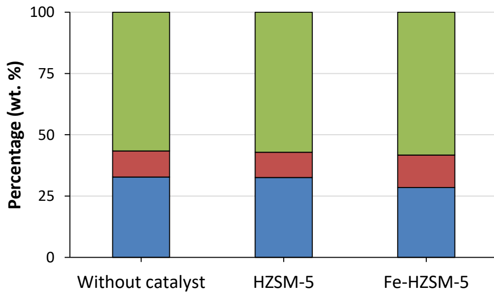
(c) Lignin
