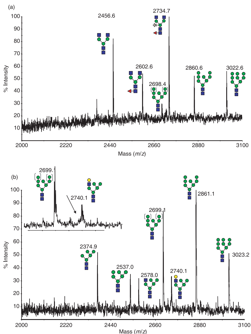
Figure 7 Matrix-assisted laser desorption ionization-time of flight-mass spectrometry (MALDI-TOF-MS) of the tryptic glycopeptides EEQFNSTFR from purified C5-1 expressed alone (a) or co-expressed with N -acetylglucosaminyltransferase I (GNTI)/β1,4-galactosyltransferase (GalT) (b). Inset presents the enlargement of m/z 2650–2800 to illustrate the absence of the main complex N -glycan ( m/z 2735 indicated by the arrow) form detected on the antibody expressed alone. N -glycan structure is shown in Figure 6.
