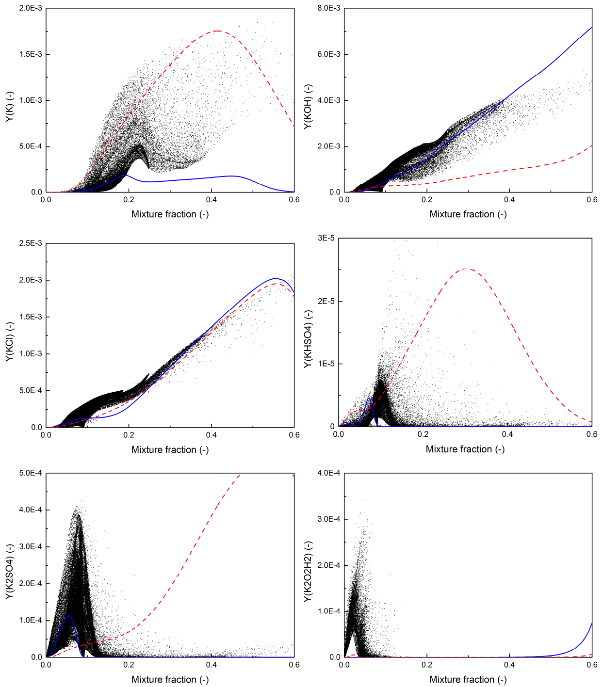
Figure 7. Scatter plots of instantaneous mass fractions of K, KCl, KOH, KHSO 4 , K 2 SO 4 and K 2 O 2 H 2 against Z at t = 20 ms. Blue solid line and red dash line are the potassium profiles obtained from 1D counterflow diffusion flames, corresponding to the lowest (21 s -1 ) and highest strain rates (8556 s -1 ).
