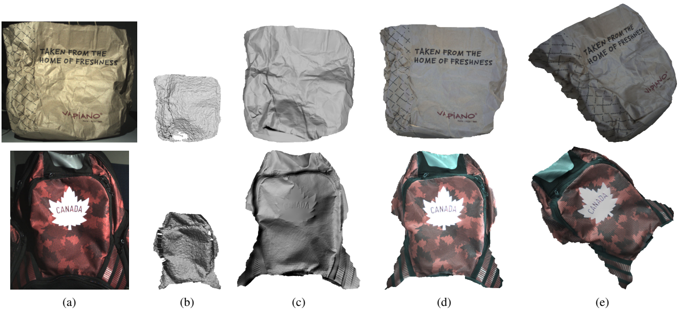
Figure 9: Qualitative results on real-world datasets. (a) One of the HR RGB images. (b) One of the LR depth maps ( SF = 4 , but the LR depth maps are enlarged for the sake of illustration). (c) Estimated HR depth map (paper bag \lambda = 40 , backpack \lambda = 10 ). (d) Estimated HR reflectance map. (e) Relighting of the HR 3D-model from new viewing and lighting angles.
