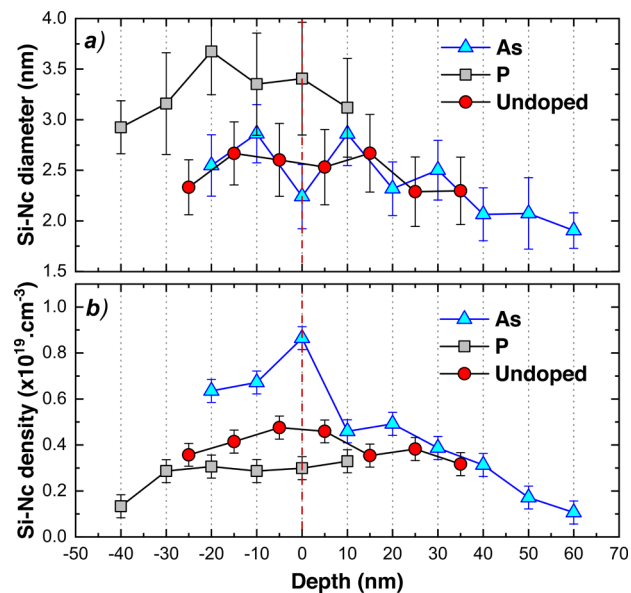
Figure 5. (a) Mean Si-Nc diameter of P-doped (gray squares), As-doped (cyan triangles), and undoped (red circles) samples and (b) density of Si-Ncs of P-doped, As-doped, and undoped samples computed in 10 nm deep boxes along the analyzed volume. The zero position represents the peak of the implantation profile.
