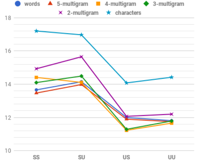
Fig. 4. WER (%) on the FR (left) and EN (right) test datasets for the four experimental setups where language models are based on large vocabularies.
