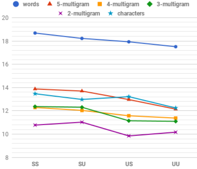
Fig. 4. WER (%) on the FR (left) and EN (right) test datasets for the four experimental setups where language models are based on large vocabularies.
