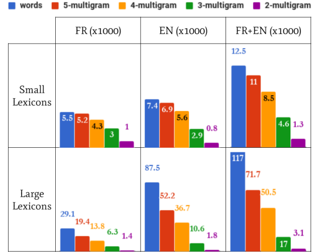
Fig. 2. Sizes of the small and large lexicons according to the lexical (words) or sub-lexical (multigrams) decomposition, on the French (FR), English (EN) and unified (FR+EN) training sets.
