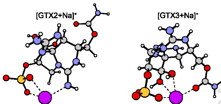
Figure 7. Representation of the sodium chelation for the lowest energy (in terms of E_{ZPE} ) optimized structures of [GTX2+Na]^+ ( E_{ZPE} = -1936.3832 E_h ) on the left and [GTX3+Na]^+ ( E_{ZPE} = -1936.3667 E_h ) on the right. Carbon atoms in grey, hydrogen atoms in white, nitrogen atoms in blue, oxygen atoms in red sulfur in yellow, and sodium atom is colored in purple.
