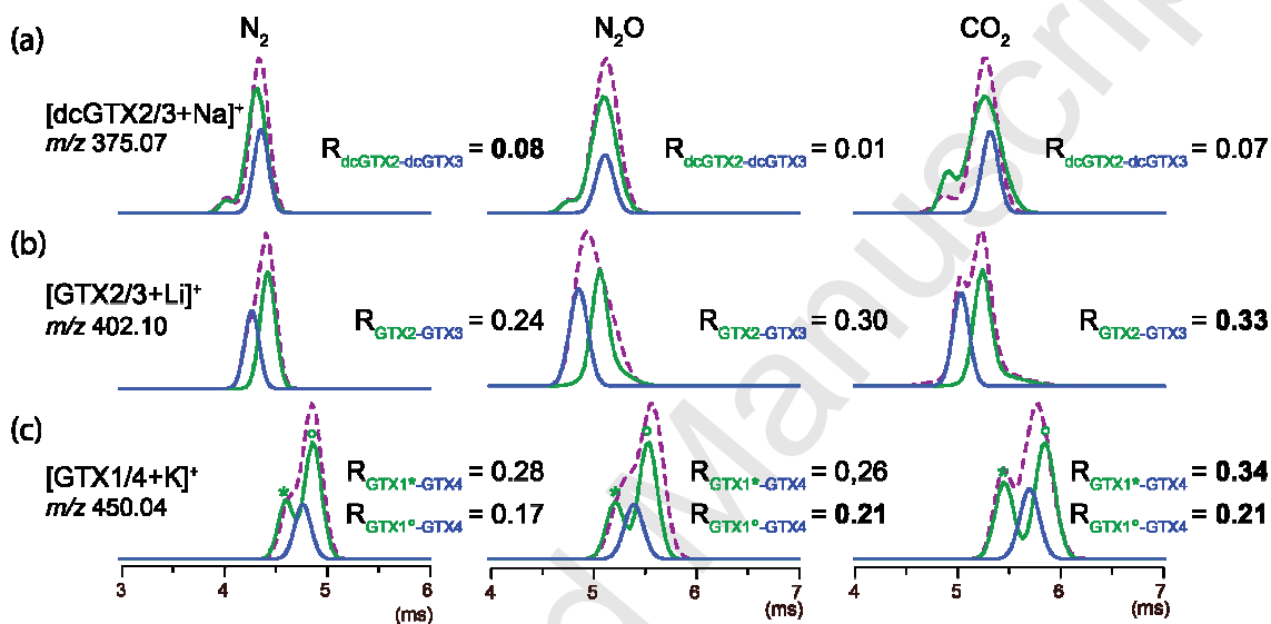
Figure 4. XIMS of [dcGTX2/3+Na] + m/z 375.07, [GTX2/3+Li] + m/z 402.10 and [GTX1/4+K] + m/z 450.04 in N 2 , N 2 O and CO 2 drift gases from IM-MS and HILIC-IM-MS. In purple dashed, XIMS obtained from mixtures in direct introduction. In green, dcGTX2, GTX2 and GTX1 (R,S,R,R); in blue, dcGTX3, GTX3 and GTX4 (R,S,R,S) XIMS extracted from HILIC-IM-MS experiments.
