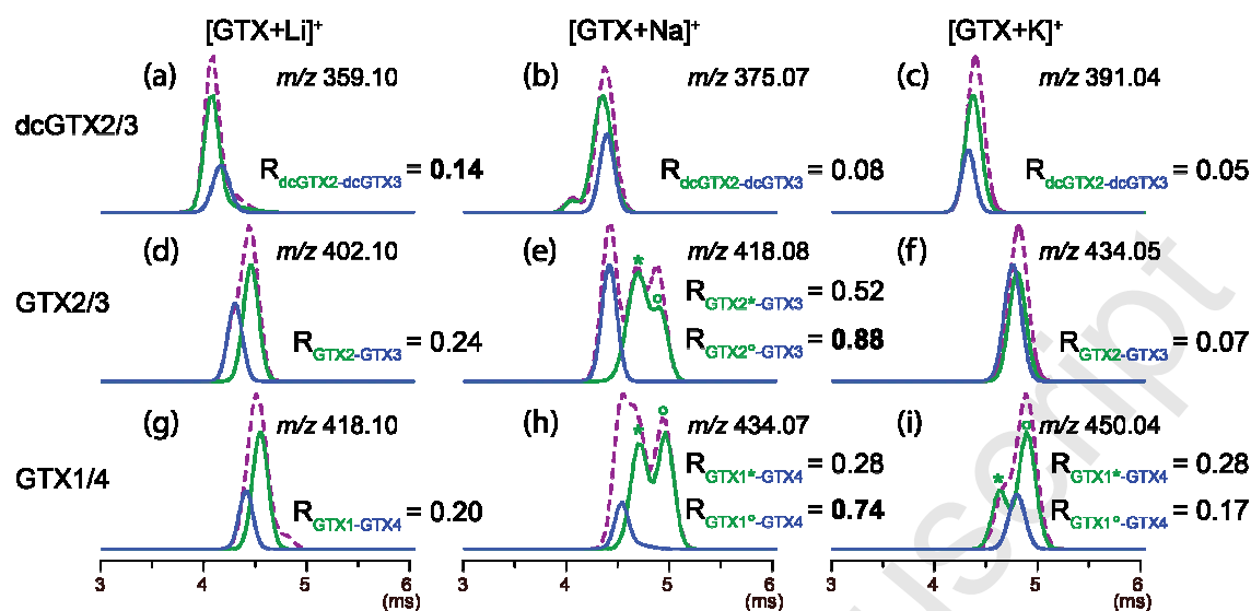
Figure 3. Ion mobility spectra observed in N_2 in the following conditions: wave velocity 800 \text{ m s}^{-1} , height wave 40 \text{ V} and gas flow 90 \text{ mL min}^{-1} . Green XIMS correspond to dcGTX2, GTX1 or GTX2 (R,S,R,R), extracted from HILIC-IM-MS experiments and blue XIMS to dcGTX3, GTX4 or GTX3 (R,S,R,S). Purple dashed XIMS correspond to the mixtures of diastereomers of dcGTX2/3, GTX1/4 or GTX2/3, extracted from direct infusion experiments.
