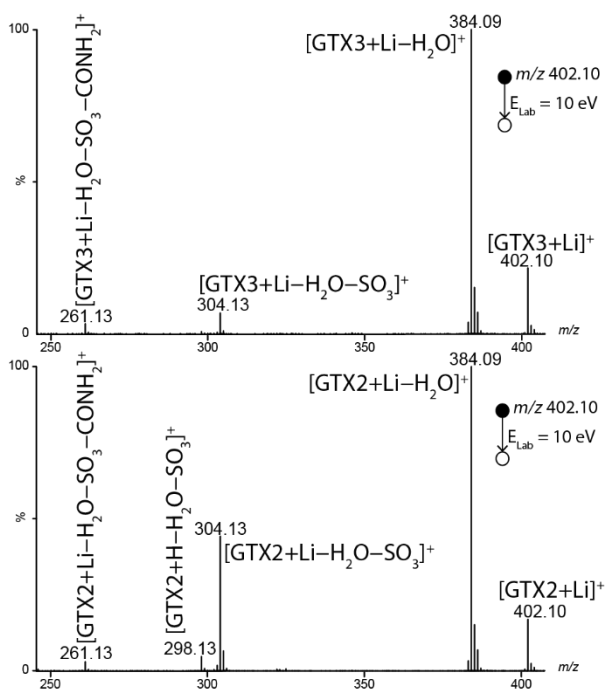
Figure S2. MS/MS spectra using 10 V of activation energy in the trap cell of lithiated GTX2 and GTX3 extracted from HILIC-MS experiment with a background subtraction. A solution of LiI at 1 mmol L -1 adjusted at pH 3.5 with formic acid was used as aqueous mobile phase.
