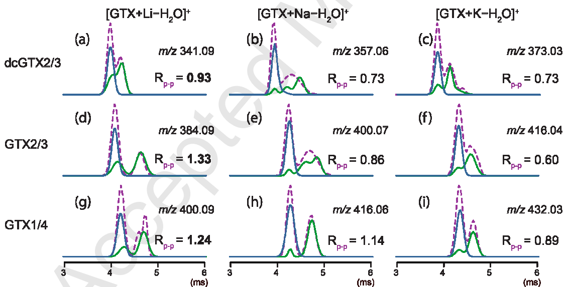
Figure 5. XIMS observed in \text{N}_2 using 10 eV collision energy in the trap cell for [\text{GTXs}+\text{Li}-\text{H}_2\text{O}]^+ and [\text{GTXs}+\text{Na}-\text{H}_2\text{O}]^+ product ions, 20 eV for [\text{GTXs}+\text{K}-\text{H}_2\text{O}]^+ . Green XIMS correspond to dcGTX2, GTX1 or GTX2 (R,S,R,R), and blue XIMS to dcGTX3, GTX4 or GTX3 (R,S,R,S) from HILIC-IM-MS/MS experiments. Purple dashed XIMS correspond to the mixtures of diastereomers of dcGTX2/3, GTX1/4 or GTX2/3, extracted from IM-MS/MS experiments. R_{p-p} are calculated from direct introduction experiments, bold values correspond to highest resolution of separation.
