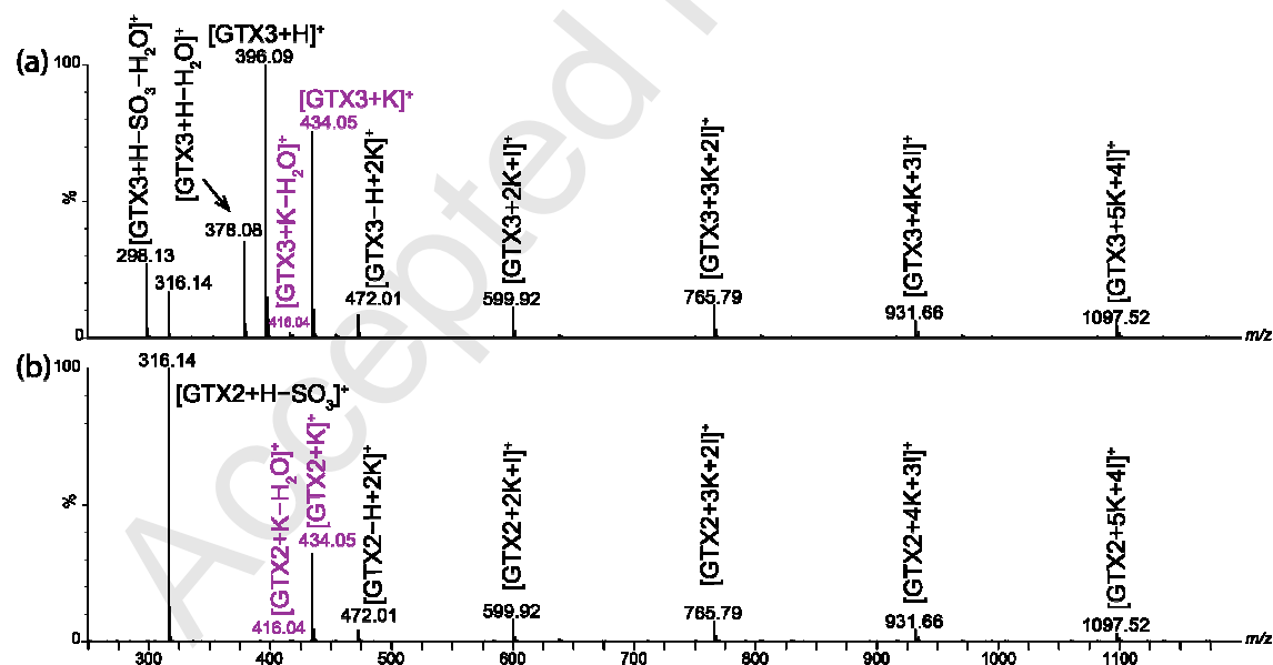
Figure 1. Mass spectra of GTX3 (a), GTX2 (b) extracted from LC-MS experiments. Solvent A: aqueous solution of KI at 1 \text{ mmol L}^{-1} , adjusted to pH 3.5 with formic acid, and solvent B: acetonitrile, were used as mobile phase.
