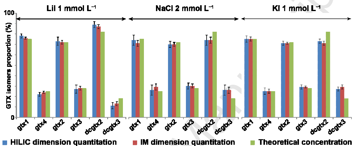
Figure 2. Relative proportions of GTX isomers determined from HILIC-IM-MS experiments using salt addition in the mobile phase in the concentration range for GTXs of 1-20 \mu\text{mol L}^{-1} . Error bars correspond to twice the standard deviation value for n=8 experiments.
