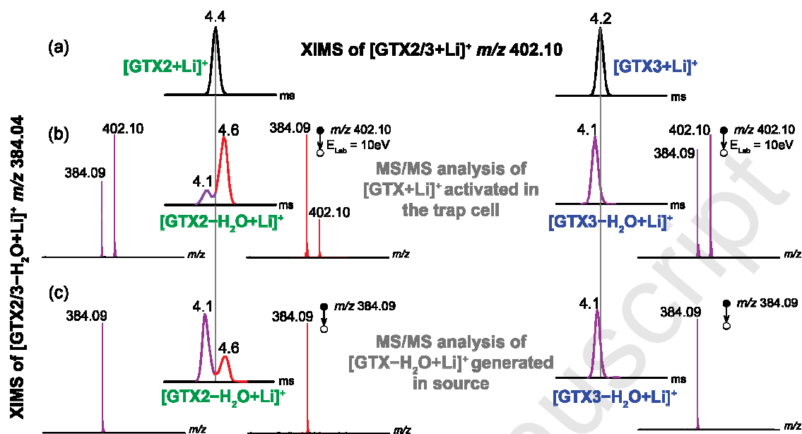
Figure 6. (a) XIMS of [\text{GTX2/3+Li}]^+ , (b) IM separation of [\text{GTX2/3-H}_2\text{O+Li}]^+ generated from [\text{GTX2/3+Li}]^+ after activation in the trap cell of the instrument, and (c) IM separation of [\text{GTX2/3-H}_2\text{O+Li}]^+ generated in source and selected in the quadrupole.
