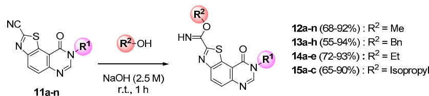
Scheme 4. General synthesis of carbimides 12 , 13 , 14 and 15 from 11 series (for yields see Table 2).
