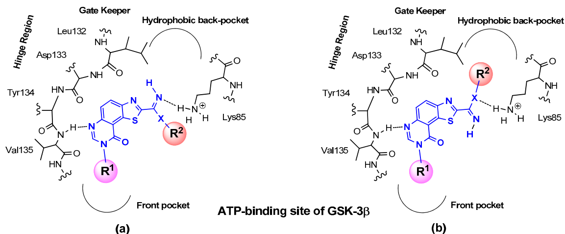
Figure 3. Suggested position of envisioned molecules in the targeted binding sites (example of the ATP-binding site of GSK-3 \beta ): (a) cis - spatial position of R^1 and R^2 or (b) trans -spatial position of R^1 and R^2 .
