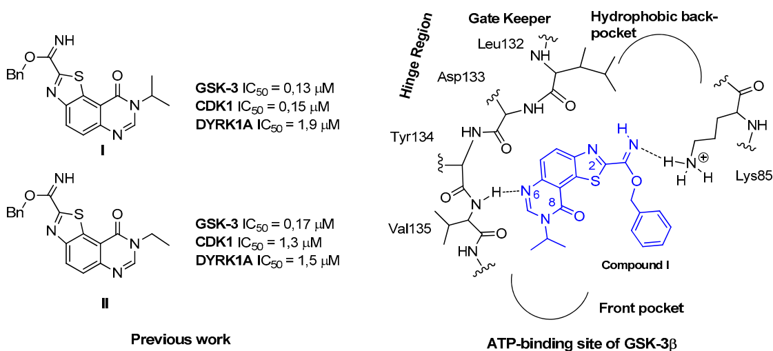
Figure 2. Schematic representation of the proposed binding mode of compound I in the ATP-binding site of GSK-3β.
