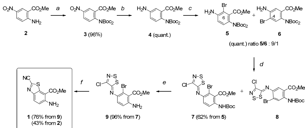
Scheme 2. Multistep synthesis of the key benzothiazole 1 . Reagents and conditions: (a) \text{Boc}_2\text{O} (2.3 equiv), DMAP (1.0 equiv), \text{Et}_3\text{N} (1.0 equiv), THF, r.t., 5 h; (b) \text{HCO}_2\text{NH}_4 (5.0 equiv), Pd/C (10%), EtOH, 78 °C ( \mu\text{w} ), 15 min; (c) NBS (1.0 equiv), DMF, -10^\circ\text{C} , 3 h; (d) Appel salt (1.2 equiv), Py. (2.3 equiv), \text{CH}_2\text{Cl}_2 , r.t., 3 h; (e) TFA, \text{CH}_2\text{Cl}_2 , r.t., 2 h; (f) CuI (1.0 equiv), Py., 115 °C ( \mu\text{w} ), 30 min.
