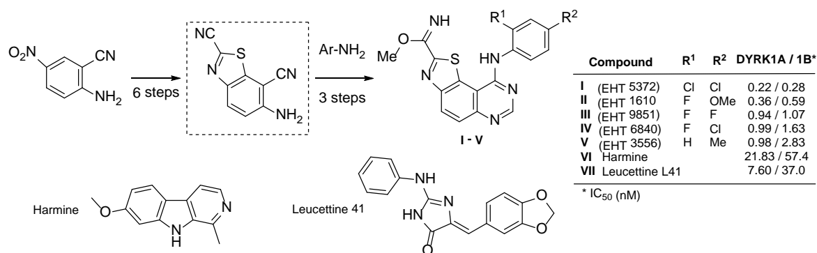
Scheme 1. 6-Aminobenzothiazole-2,7-dicarbonitrile, a versatile molecular platform for global chemistry strategy and structures of the five best DYRK1A/1B inhibitors. Harmine and Leucettine 41 (L41) are positive control inhibitors.
