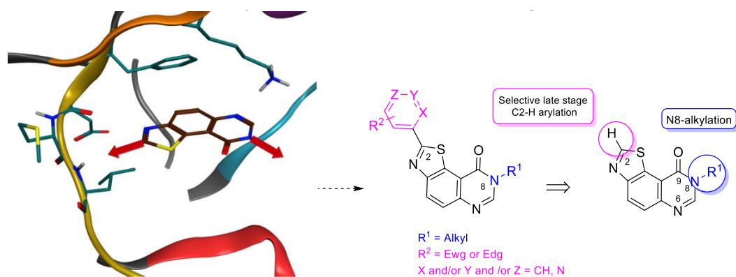
Scheme 3. Fragment-growing anchor points envisioned on the thiazolo[5,4- f ]quinazolin-9(8 H )-one scaffold ( left ). Schematic representation of the predicted binding modes and retrosynthetic route to C2-arylated derivatives suggested via C–H arylation of the former C2-H thiazole precursor ( right ).
