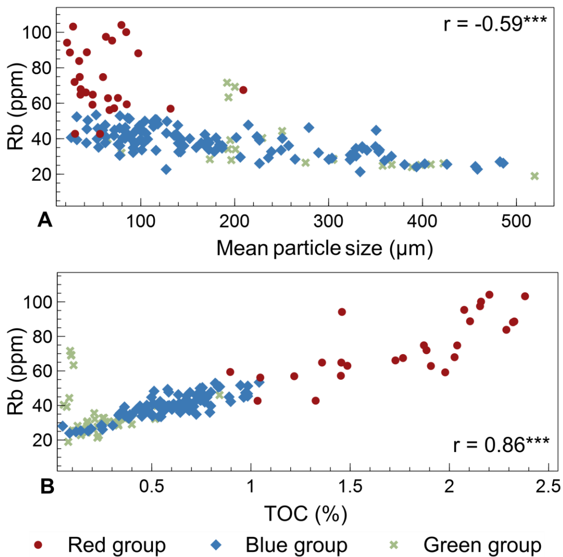
Fig. 5: A: Relation between Rb (ppm) and mean particle size ( \mu\text{m} ) for the three groups identified in figure 3; B: Relation between Rb (ppm) and TOC (%) for the three groups identified in figure 3.
