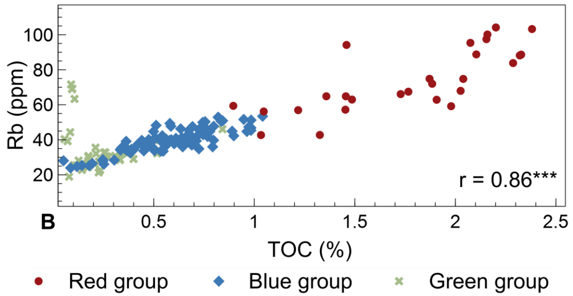
Fig. 5: A: Relation between Rb (ppm) and mean particle size (µm) for the three groups identified in figure 3; B: Relation between Rb (ppm) and TOC (%) for the three groups identified in figure 3.
