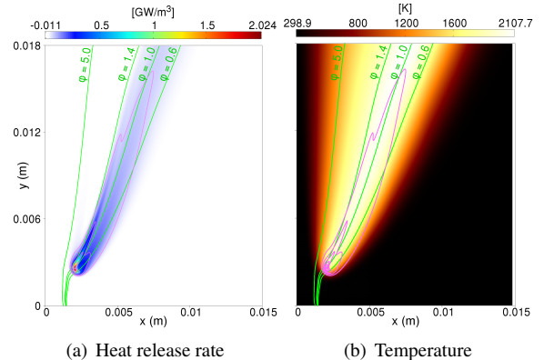
Figure 4: Edge flame simulated with the FTC solver. In green: isolines of Z corresponding to \phi = 0.6, 1.0, 1.4 and 5.0 . In pink: isolines of heat release rate (0.05, 0.2, 0.5, 1.0, 1.5 and 2.0 \text{ GW/m}^3 ).
