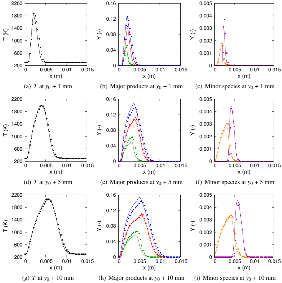
Figure 9: Radial profiles of temperature (black), major products (CO in green, CO 2 in red and H 2 O×1.2 in blue) and minor species (OH in purple and H 2 in orange) at different heights above the flame tip ( y_0 ), for the FTC (symbols) and HTTC (lines) simulations.
