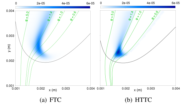
Figure 8: Mass fraction of C_2H_5 (zoom) computed Z and Y_c = Y_{CO} + Y_{CO_2} . Green: isolines of \phi . Black: isoline of Y_c = 0.005 .
