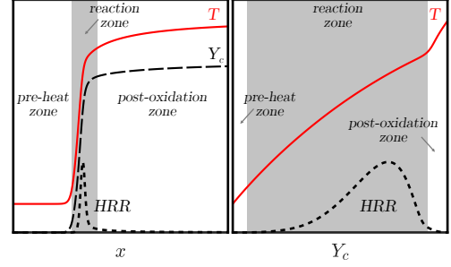
Fig. 1: General characteristics of premixed flamelets - left: Temperature, progress variable and heat release rate (HRR) in physical space. Right: Temperature and heat release rate (HRR) in progress variable space. In comparison to the physical space, the reaction zone is enlarged in progress variable space, while pre-heat zone and post-oxidation zone are confined to thin layers at the boundaries.
