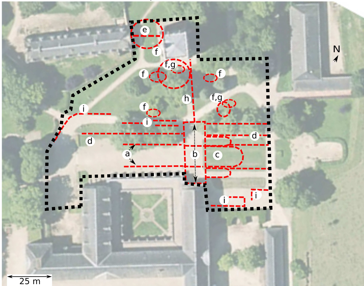
Figure 11: Sketch of the main geophysical anomalies (in red-dashed line). In black-dotted line, the prospected area as depicted in the Figure 3.
