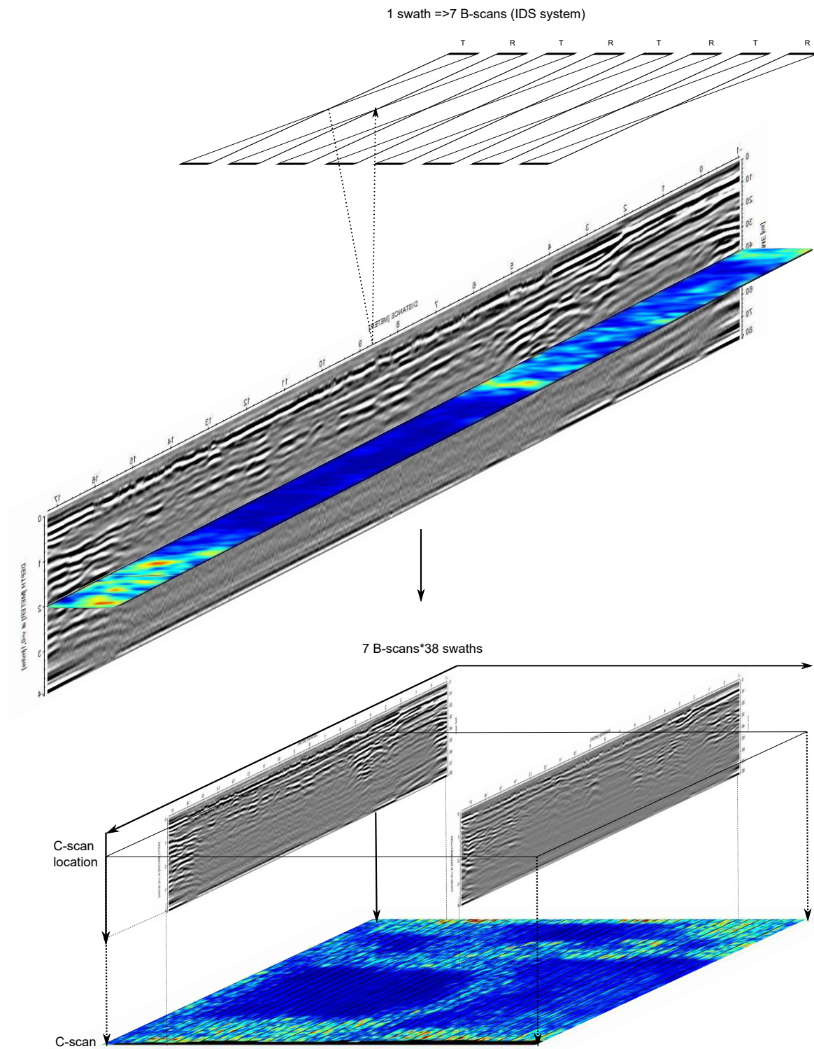
Figure 4: 3D-GPR principle, from B-scan, C-scan to GPR map (inspired from Ranieri et al. (2015)).
