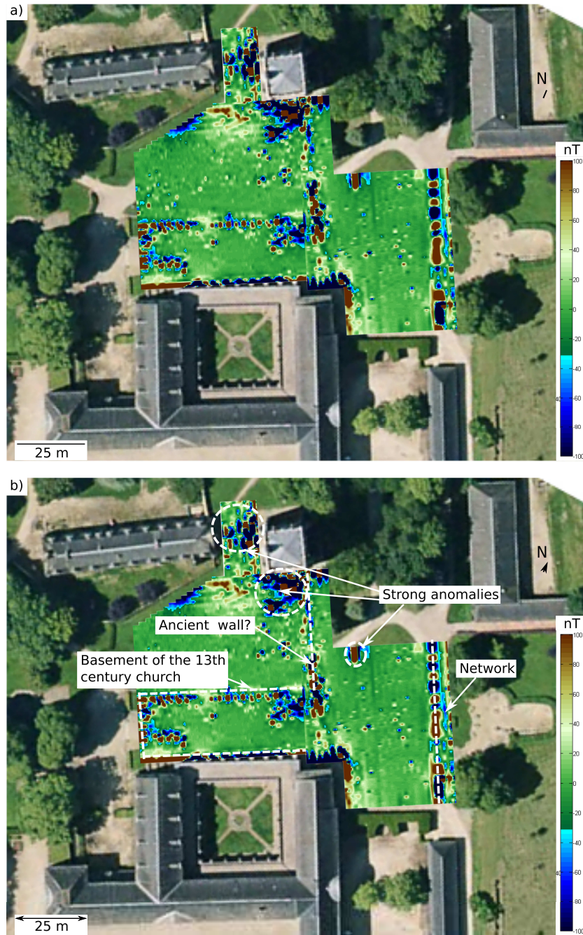
Figure 7: a) Raw magnetic survey and b), interpreted anomalies.
