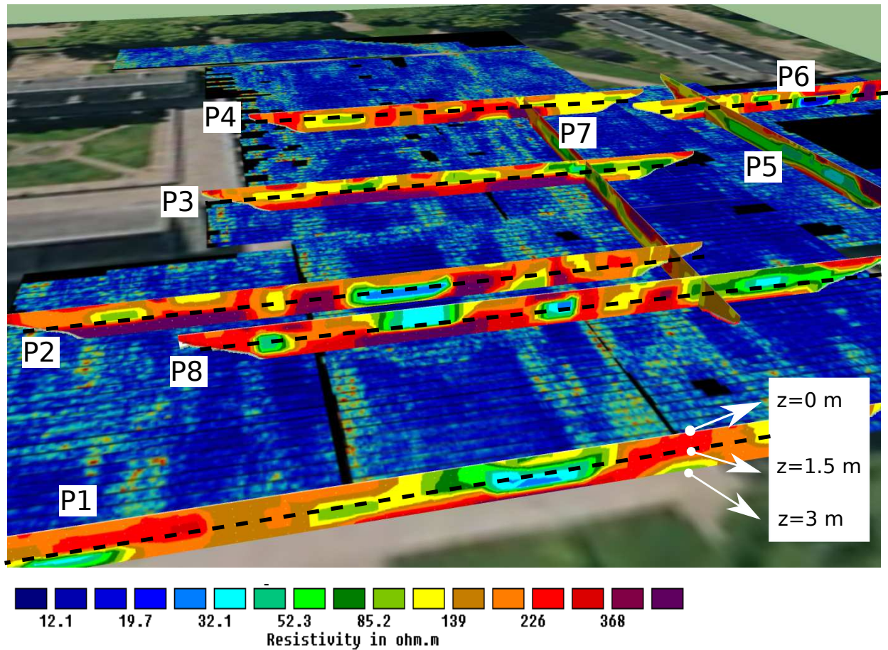
Figure 9: Superimposition of 8 Wenner images and the radar slice at 1.5 m depth. The black-dashed lines reported on each resistivity image is the 1.5 m depth of the radar slice.
