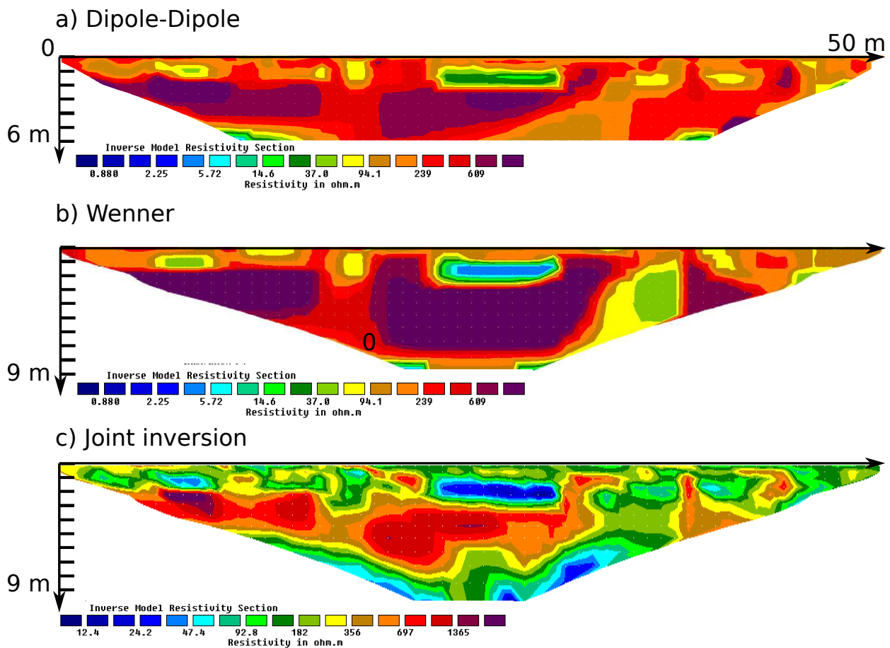
Figure 8: Comparison of IRE profile P2, a) Dipole-Dipole, b) Wenner and c) Joint inversion of Wenner and Dipole-Dipole data.
