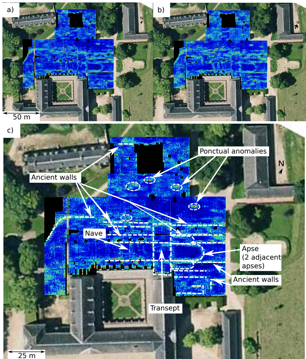
Figure 6: a) GPR slices at 1 m depth and b), at 2 m depth. c) Interpreted anomalies.
