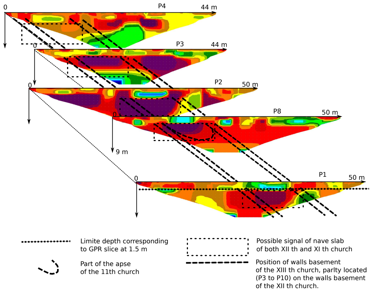
Figure 10: 5 Wenner profiles (P1-4 and P8) and sketch of the apse of the original Romanesque church surrounding by two longitudinal features that correspond to the walls basement of the 11th till P8, and to the walls basement of 13th church beyond.
