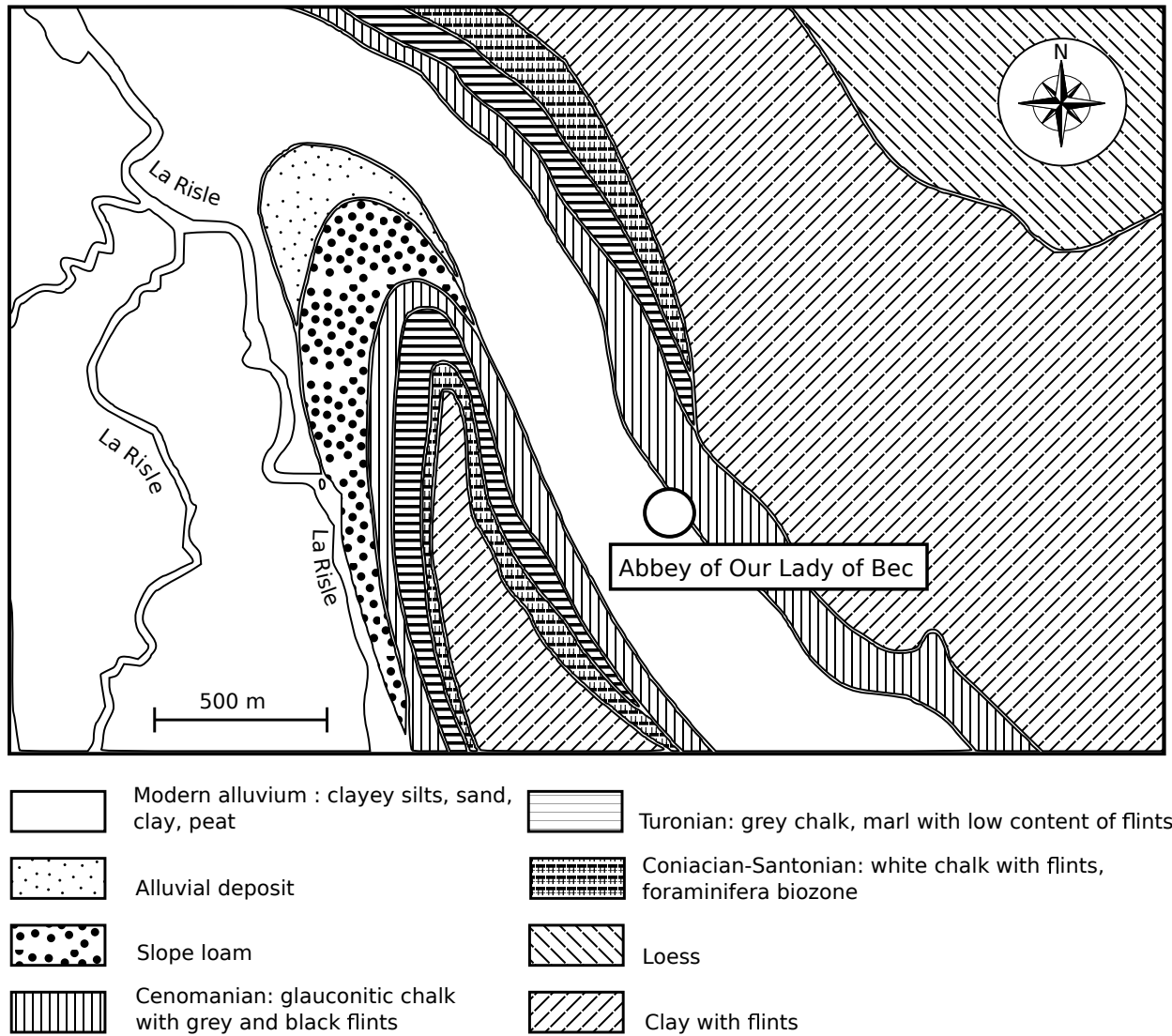
Figure 2: Geological map of the Abbey of Our Lady of Bec. The first centimeters of the shallow surface is mainly composed of anthropogenic materials and modern alluvium.
