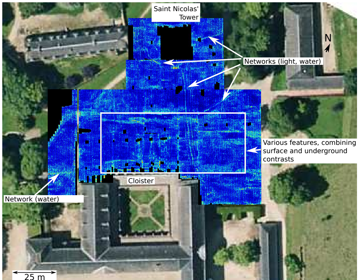
Figure 5: GPR slice at 0.3 m depth.
