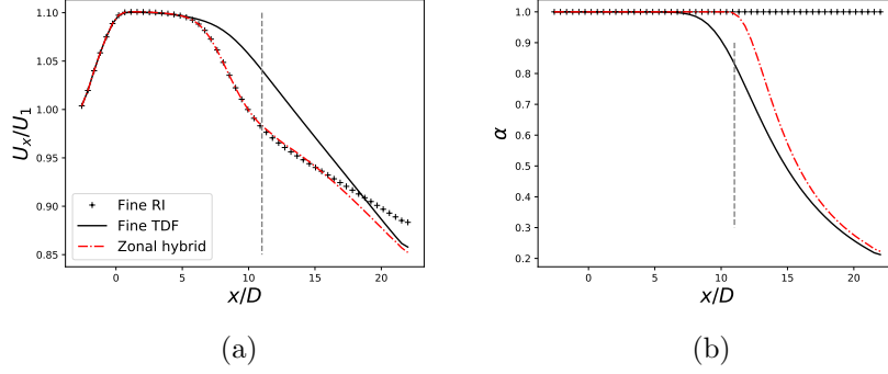
Figure 11: Steady state (a) velocity and (b) liquid volume fraction profiles along jet center line. Zonal domain interface \Gamma at x = 11D is indicated by a vertical dashed line.
