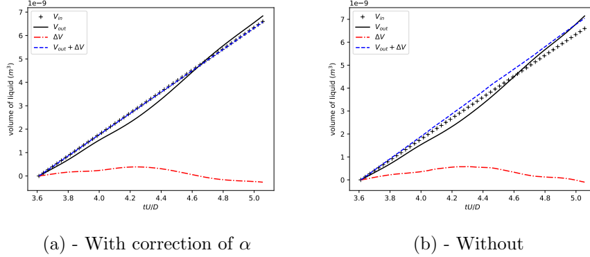
Figure 18: Evolution of volume of liquid in the medium zonal hybrid simulation.
