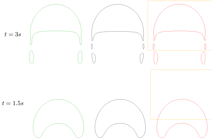
Figure 6: Interface ( \alpha = 0.5 ) at (a) t = 1.5s and (b) t = 3s for three simulations of Hysing skirted bubble configuration [36]. From left to right, the green line is the coarse mesh, the black line is the fine mesh and the red line is the coarse mesh coupled with a fine zonal mesh. The zonal interface \Gamma is shown with an orange rectangular box.
