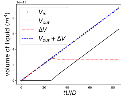
Figure 12: Evolution of volume of liquid using the zonal grid solver.
