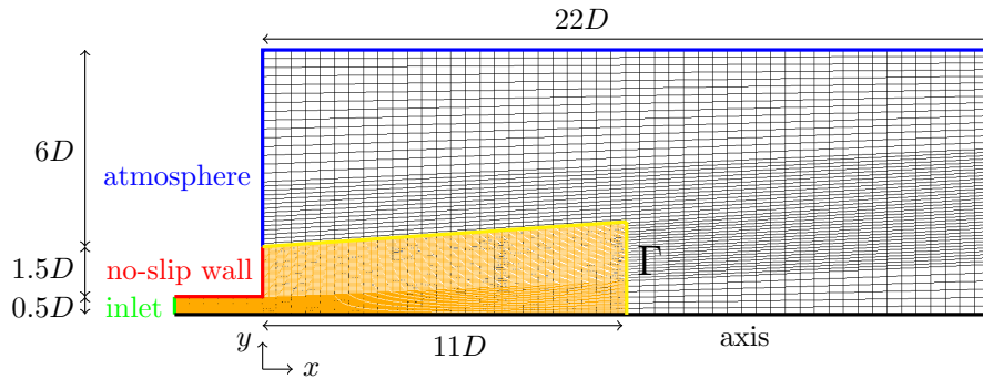
Figure 8: Configuration of the liquid-air jet configuration. The zonal domain (ZD), with fine refinement, is shown in yellow. The main (global) domain (GD), with coarse refinement, is shown in black. \Gamma stands for the zonal domain interface with the global domain and is indicated by the yellow line.
