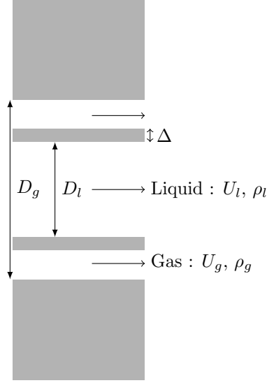
Figure 13: Schematic of the injector used by Stepowski et al. [37].
