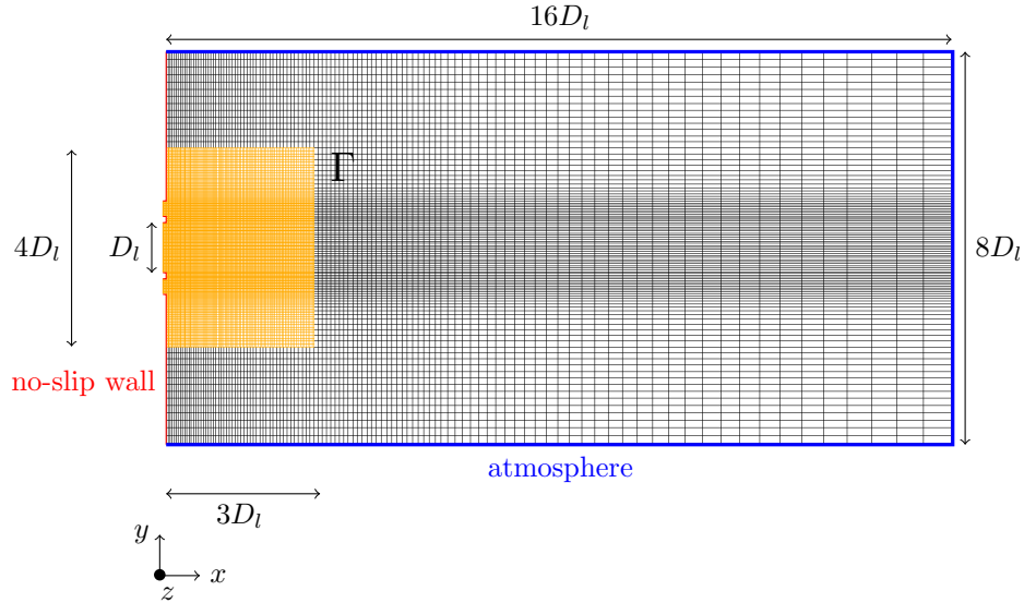
Figure 14: Dimensions and boundary conditions of the 3D computational domain. The zonal domain, with medium refinement, is shown in yellow. The global domain, with coarse refinement, is shown in black. \Gamma stands for the zonal interface with the global domain.
