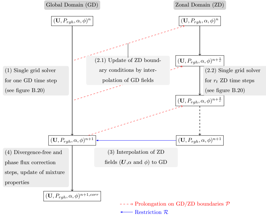
Figure 2: Zonal methodology algorithm; r_t is the time refinement ratio between ZD and GD. \mathbf{U} is the velocity field, P_{rgh} is the pressure field, \alpha the primary phase field and \phi a transported scalar quantity field. Subscript ()^n is the index for time instant t and ()^{n+1} stands for the time instant t + \Delta t after one time step.
