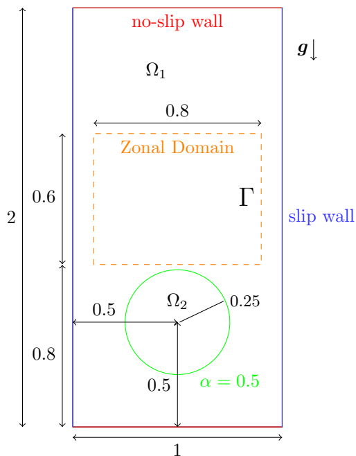
Figure 5: Simulation domain, boundary conditions and initial configuration of Hysing et al. [36] rising bubble problem. The zonal domain, with interface \Gamma , is placed above the initial position, with a mesh refinement of 2 : 1.
