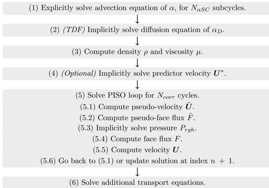
Figure B.20: Algorithm structure of both single grid two-phase solvers.
