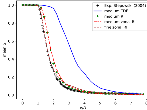
Figure 17: Mean liquid volume fraction axial profiles, along the injector central axis. The vertical gray dashed line stands for the zonal grid interface \Gamma .
