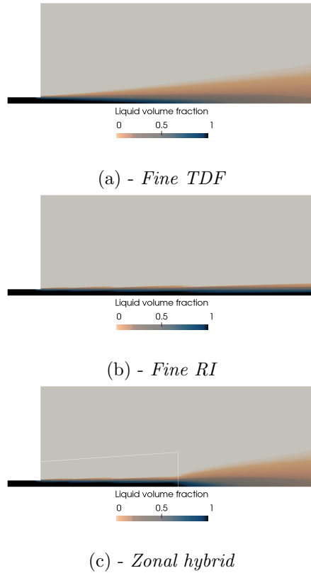
Figure 10: Steady state liquid volume fraction fields. The zonal domain interface \Gamma is indicated by a white line.
