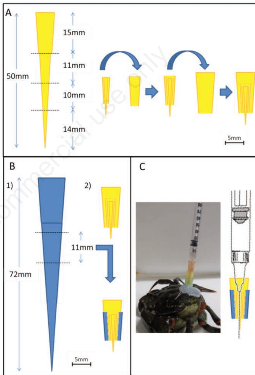
Figure 1. Injection device: graphical depiction of fabrication using 200 \mu L and 1000 \mu L pipette tips. A) Cutting and assembly of parts derived from the 200 \mu L tips. B) 1. Withdrawal of an 11 mm middle section from a 1000 \mu L tip and 2. completion of the injection device. C) Shore crab equipped with injection device fixed with epoxy on his carapace and schematic representation of the inserted syringe.
