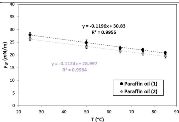
Fig. 8. Surface tension vs. temperature for paraffin oils. (For interpretation of the references to color in this figure legend, the reader is referred to the web version of this article.)
