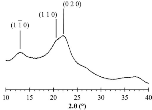
Fig. 6. X-ray diffraction pattern of the cellulosic film.
