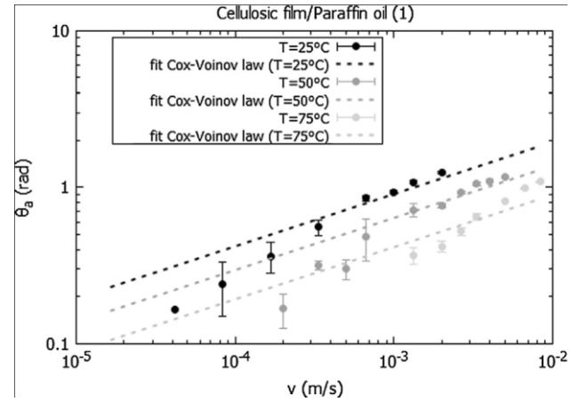
Fig. 11. Fits of experimental data of \theta_a vs. v according to the Cox-Voinov model.
