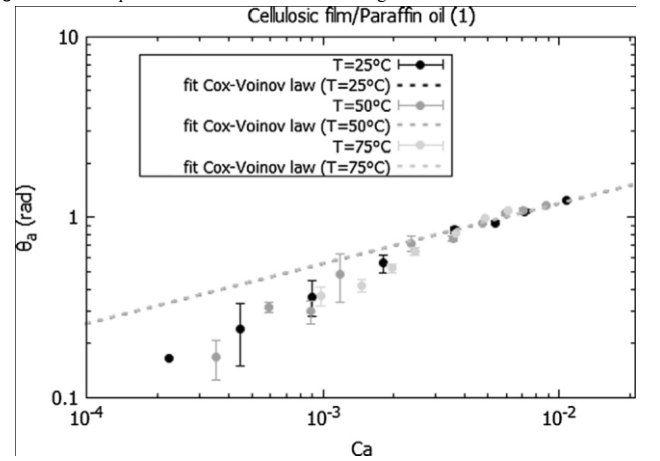
Fig. 12. Fits of experimental data of \theta_a vs. Ca according to the Cox-Voinov model.
