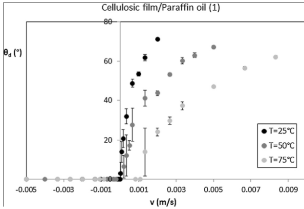
Fig. 9. Dynamic contact angles as a function of velocity for paraffin oil (1).
