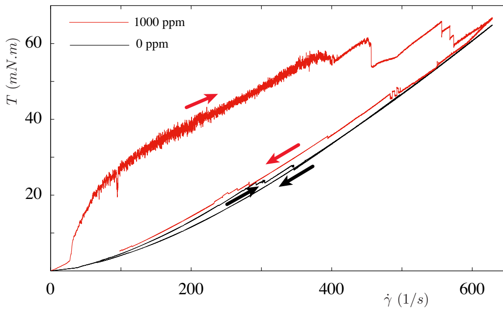
Figure 2: Torque as a function of shear rate for 0 and 1000 ppm of PEO dissolved in 7% PEG aqueous solution during an acceleration and deceleration cycle in the Taylor-Couette geometry. These experiments were done without pre-shear. The up- and down-arrows indicate the acceleration and deceleration, respectively.
