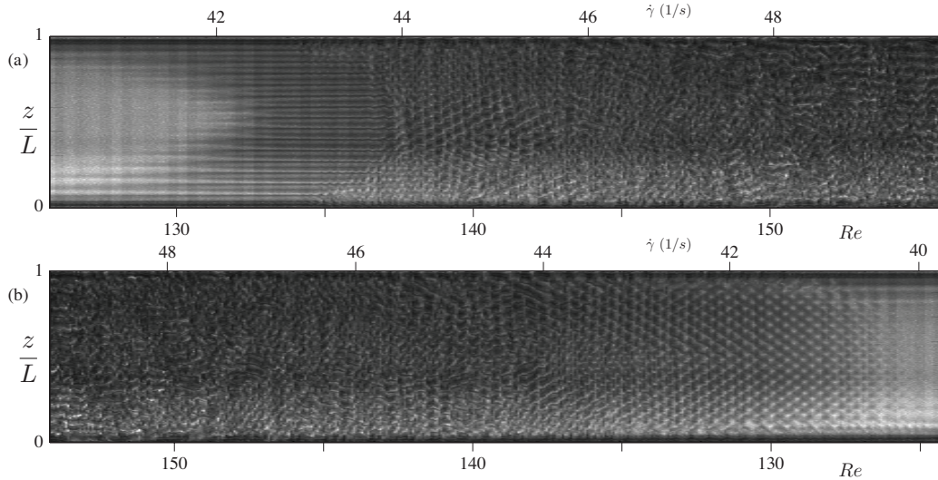
Figure 5: Spatio-temporal diagrams at the mid-plane of the gap over the whole height of the flow for 76 ppm of PEO dissolved in 7% PEG aqueous solution. (a) and (b) spatio-temporal diagrams of the flows solution during acceleration and deceleration, respectively.
