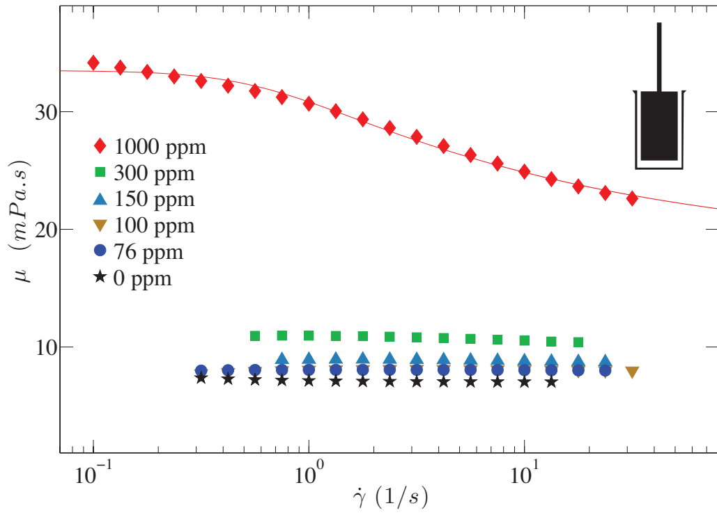
Figure 3: Shear viscosity, \mu , as a function of the shear rate, \dot{\gamma} , for different concentrations of PEO in 7% PEG aqueous solution in the bob-cup geometry. The red continuous line corresponds to a fit by the Carreau model.
