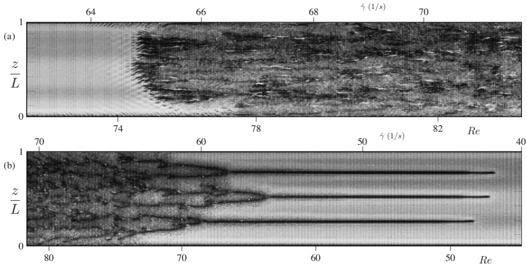
Figure 6: Spatio-temporal diagrams at the mid-plane of the gap over the whole height of the flow for 1000 ppm of PEO dissolved in 7% PEG aqueous solution. (a) and (b) spatio-temporal diagram of the flow during acceleration and deceleration, respectively. In (b) the black horizontal lines ( 56 > \dot{\gamma} > 42 1/s or 64 > Re > 48 ) correspond to diwhirls.
