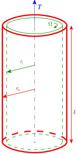
Figure 1: Schematic diagram of the Taylor-Couette experiment (drawn to scale).
