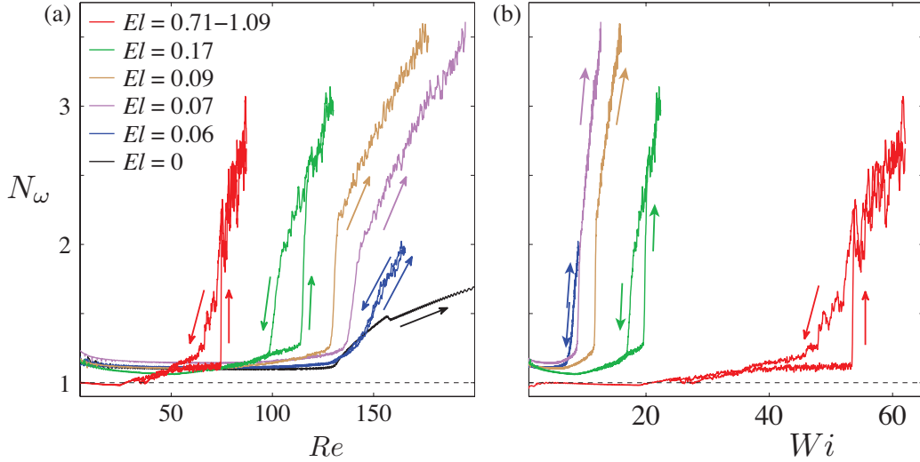
Figure 7: (a) N_\omega as a function of the Re and (b) N_\omega as a function of the Wi for solutions with different El or concentrations of PEO dissolved in 7% PEG aqueous solution. The up- and down-arrows indicate the acceleration and deceleration, respectively. Down-curves for El = 0.07 and 0.09 are omitted.
