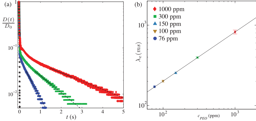
Figure 4: (a) Time evolution of the dimensionless diameter, D(t)/D_0 , for different concentrations of PEO in 7% PEG aqueous solution. The black stars correspond to the solvent. The continuous lines are fits of the thinning region in the elasto-capillary regime using (3) and dashed lines extrapolations of these fits. (b) Variation of relaxation time, \lambda_e , with the concentration of PEO. The error bars represent the standard deviation over three measurements and are smaller than the symbols. The black straight line is a power law fit with an exponent of 0.61.
