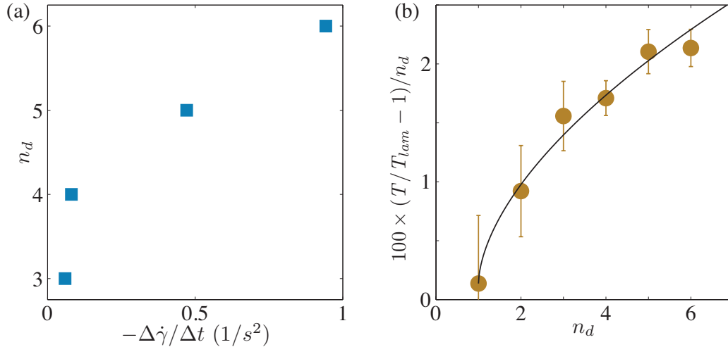
Figure 9: (a) Dependency of the numbers of diwhirls, n_d , on the deceleration of the inner cylinder, -\Delta\dot{\gamma}/\Delta t . (b) Additional dimensionless torque over the laminar per numbers of diwhirls, n_d , of flows containing six different numbers of diwhirls at Re = 51 or Wi = 37 . The black line represents a fit described in the text.
