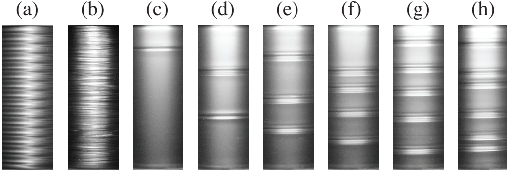
Figure 8: Snapshots over the whole height of the flow. (a) Newtonian fluid containing 30 Taylor vortices. The others are for mixtures containing 1000 ppm of PEO dissolved in 7% PEG aqueous solution and present: (b) inertio-elastically turbulent flow, (c-h) flows containing 1 to 6 diwhirls, from left to right, respectively.
