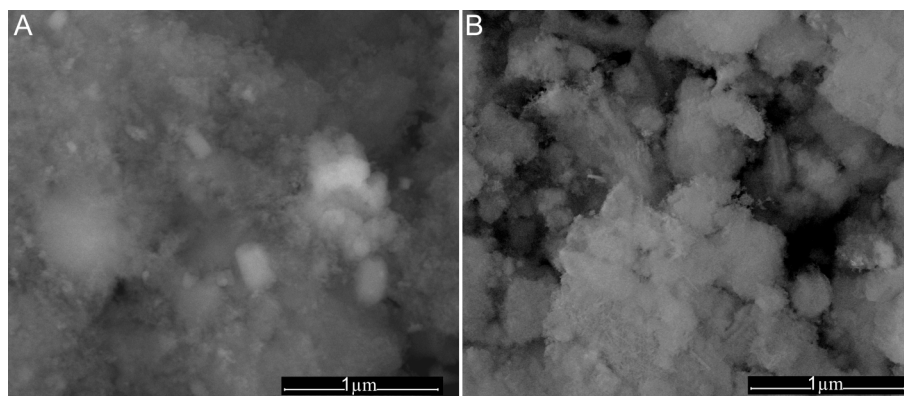
Figure 11. SEM images of: CD-HAp_1 (A); and CD-HAp_2 (B) samples after the adsorption of Pb^{2+} .
