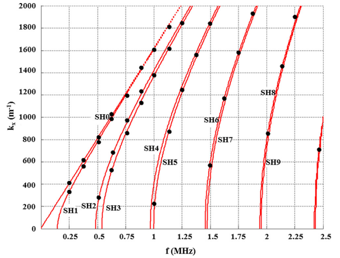
FIG. 2. (Color online) Dispersion curves of the three-layer structure (Fig. 1 and Table I): analytical method (red line), SAFE method (dots).
