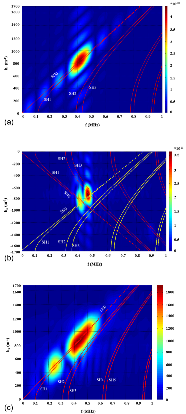
FIG. 12. (Color online) (a) 2D FFT of the incident signal (before the roughness): SH 0 incident mode. Dispersion curves of the three-layer (numerical simulation). The color amplitude is in arbitrary unit. (b) 2D FFT of the reflected signal by the roughness (before the roughness): SH 0 reflected mode. Dispersion curves of the three-layer structure and phonon curves (numerical simulation). The color amplitude is in arbitrary unit. (c) 2D FFT of the transmitted signal (after the roughness): SH 0 transmitted mode. Dispersion curves of the three-layer (numerical simulation). The color amplitude is in arbitrary unit.
