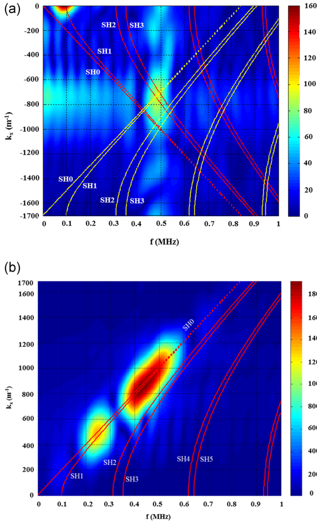
FIG. 11. (Color online) (a) 2D FFT of the reflected signal by the roughness (before the roughness): SH 2 reflected mode. Dispersion curves of the three-layer structure and phonon curves (experimental results). The color amplitude is in arbitrary unit. (b) 2D FFT of the transmitted signal (after the roughness): SH 0 transmitted mode. Dispersion curves of the three-layer structure (experimental results). The color amplitude is in arbitrary unit.
