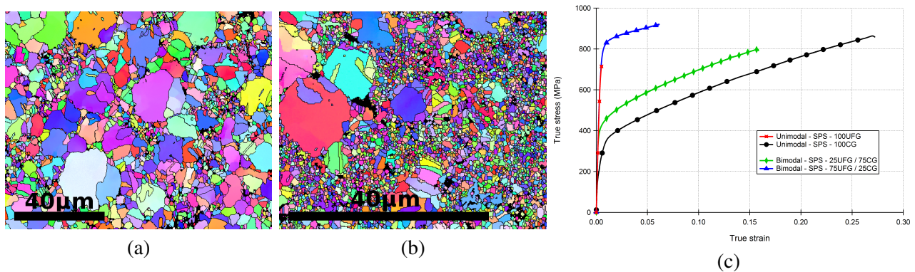
Figure 7: EBSD maps of bimodal 316L steel polycrystals elaborated by spark plasma sintering: (a) 75% 15μm-coarse-grains, 25% 0.5μm-fine-grains, (b) 25% 15μm-coarse-grains, 75% 0.5μm-fine-grains, (c) tensile responses of unimodal and bimodal 316L steel specimens elaborated by spark plasma sintering. After [6].
